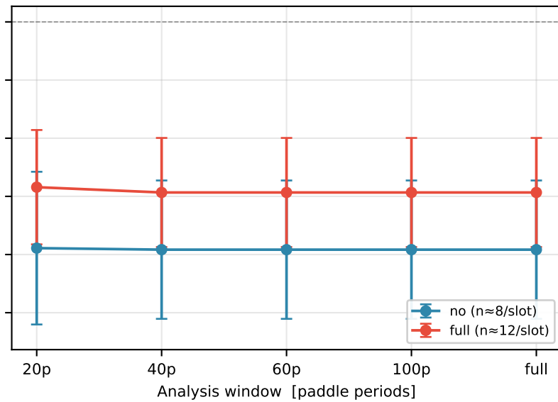
Window sensitivity | 0.20 V
