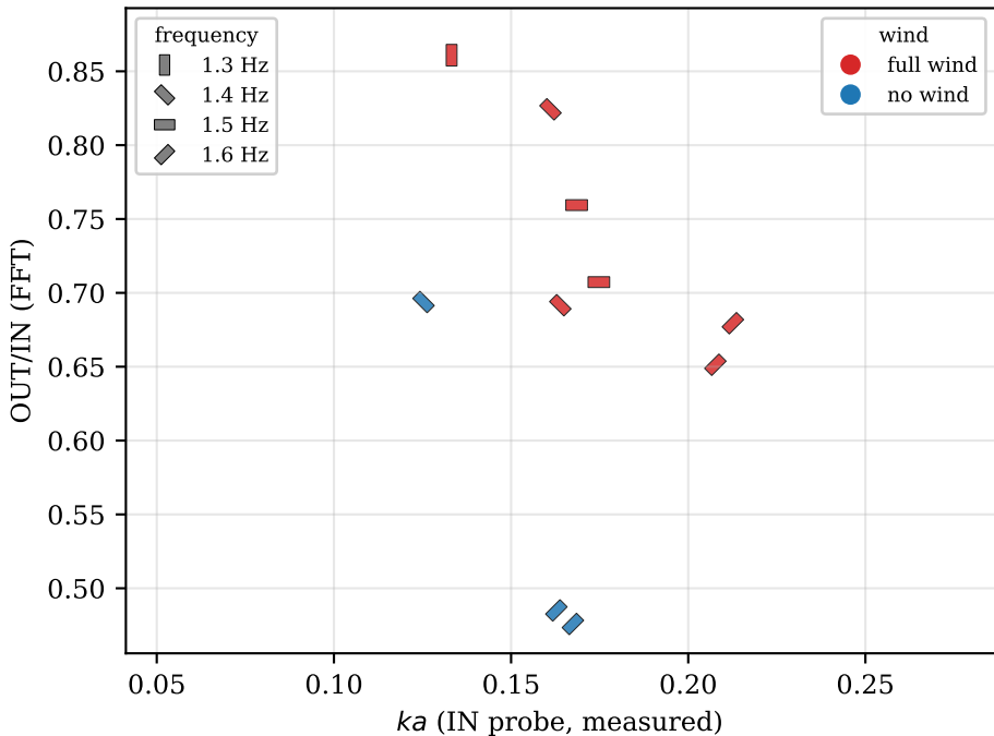
Wave transmission vs. wave steepness — full panel, 0.20 V
