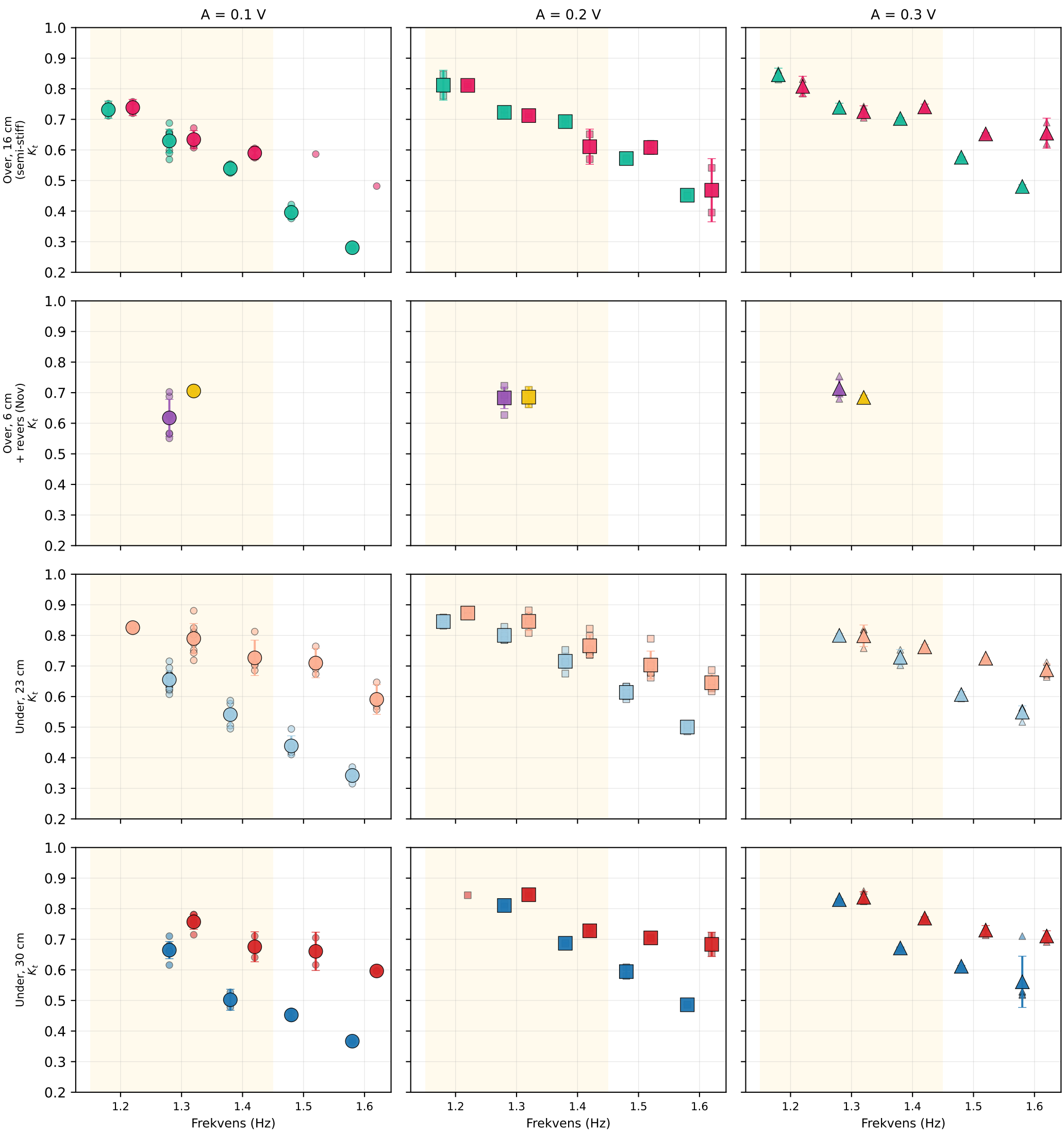
K_t vs frekvens — 4-way mooring split, color = (mooring × wind), marker = amp. Yellow band = lavfrekvens-fokus (1.2-1.4 Hz).
