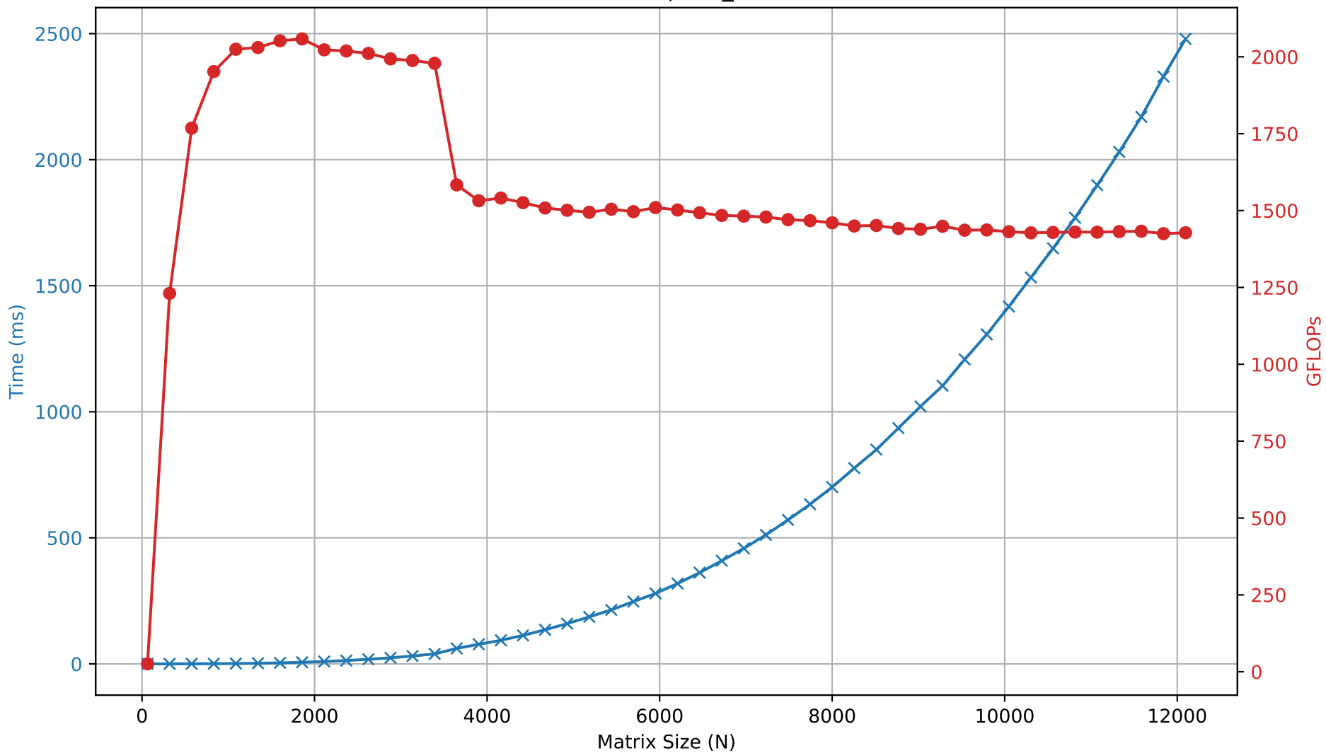
Performance: alpaka_full (float)
