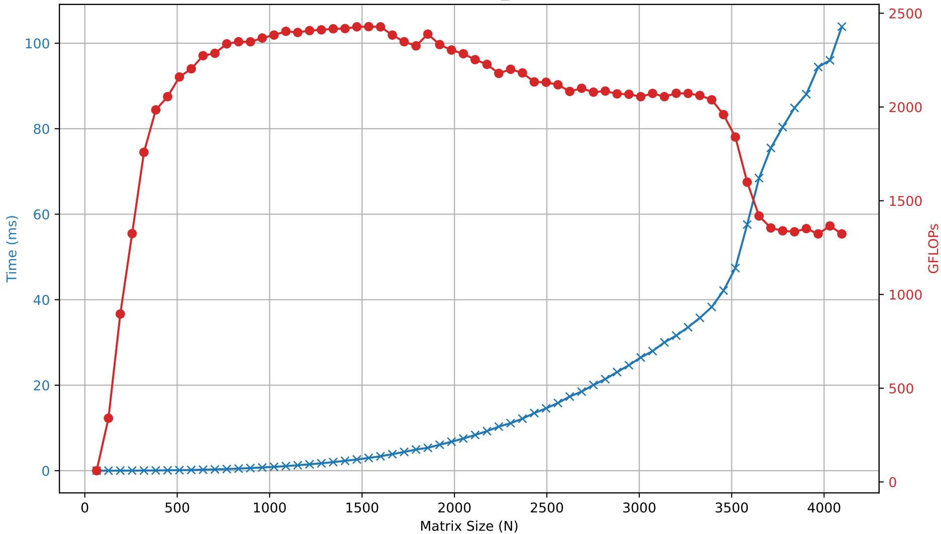
Performance: alpaka_tiling (float)
