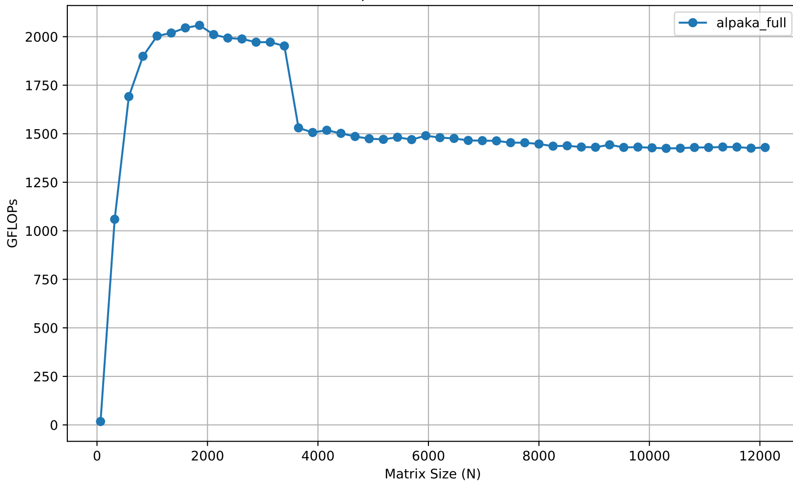
Comparison: GFLOPs (float)
