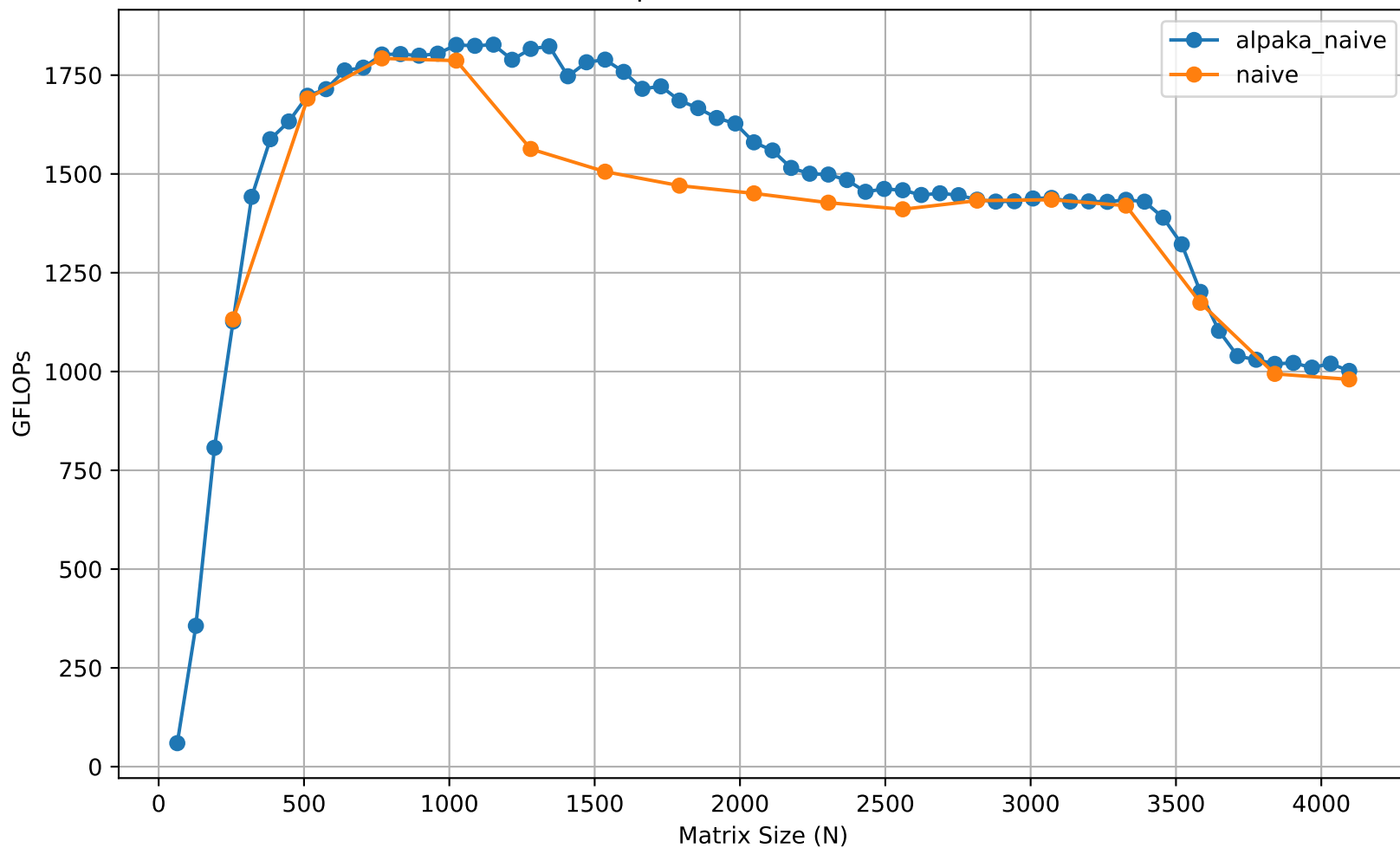
Comparison: GFLOPs (float)
