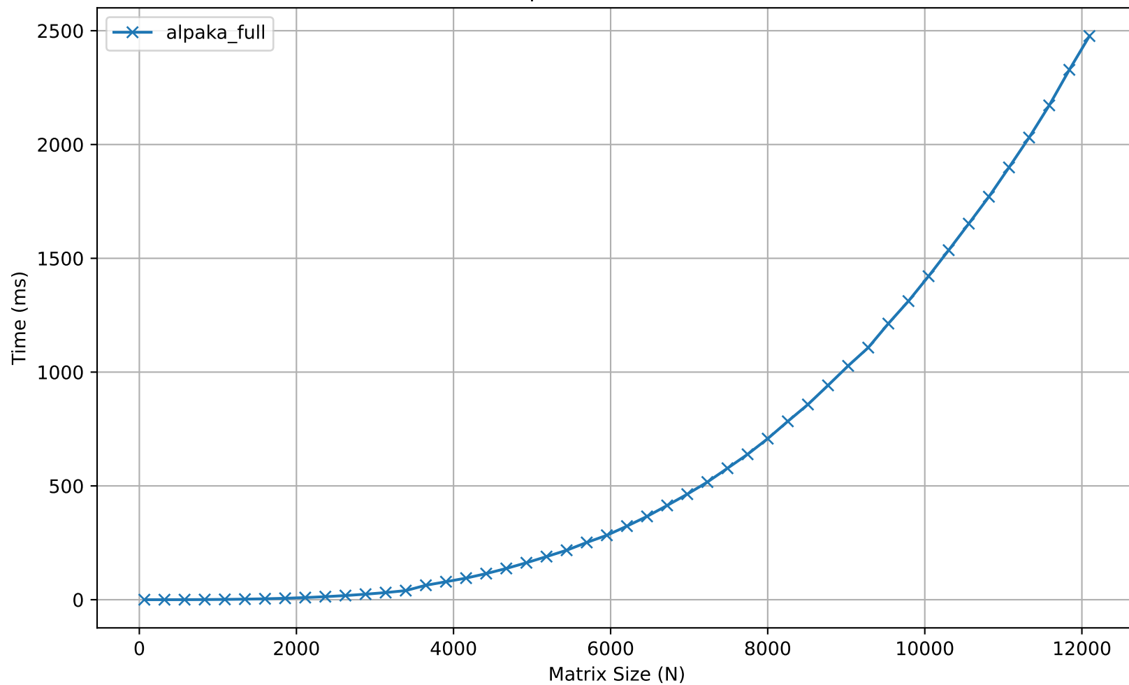
Comparison: Time (float)
