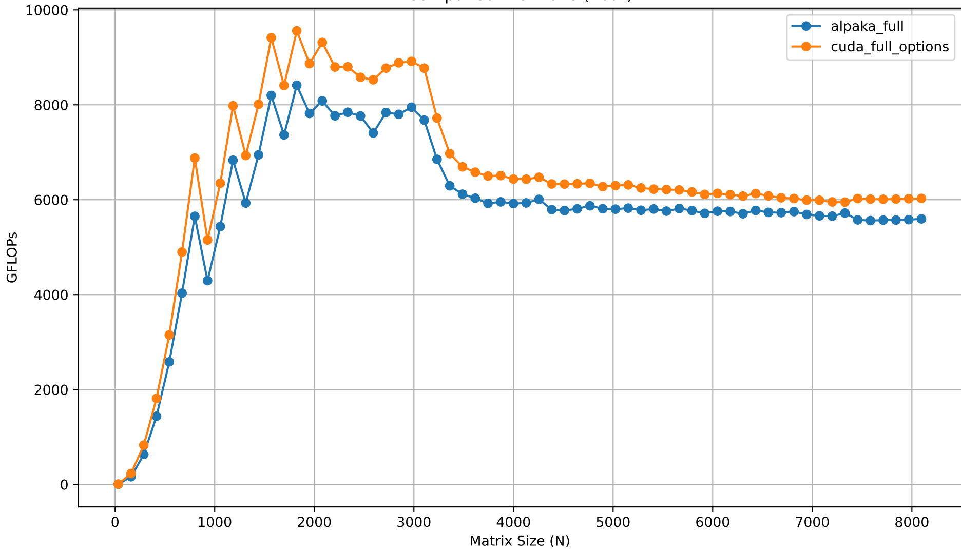
Comparison: GFLOPs (float)
