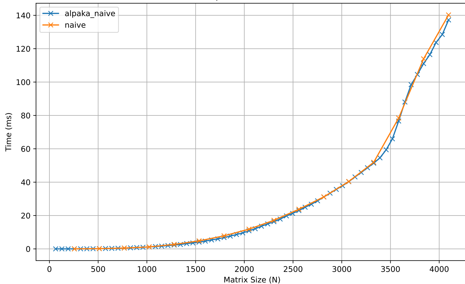
Comparison: Time (float)
