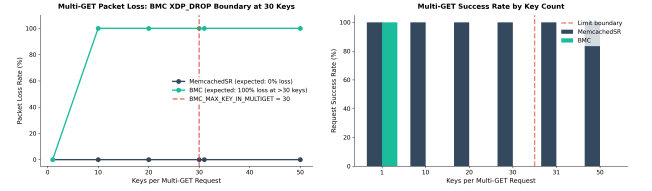
Figure 11: Packet loss rate (left) and success rate (right) vs. keys in multi-GET requests.
