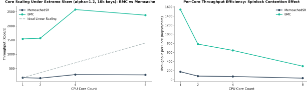
Figure 12: Open-loop throughput (left) and core efficiency (right) under Zipf \alpha = 1.2 .
