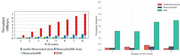
Figure 2: Open-loop core scaling comparison: original paper Figure 6 (left) and my replicated experimental results on c6525 AMD nodes (right).
