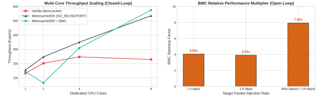
Figure 3: Throughput scaling under closed-loop memaslap workload (left) and open-loop speedup multiplier relative to Vanilla 1-core baseline under saturating flood (right).
