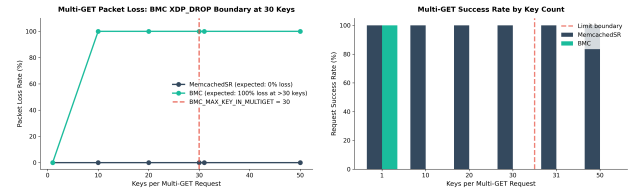
Figure 11: Packet loss rate (left) and success rate (right) vs. keys in multi-GET requests.
