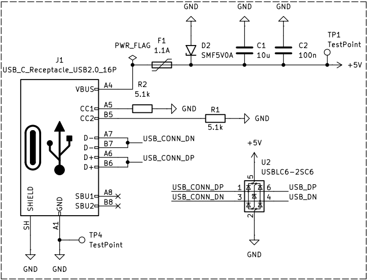
USB-C input & protection
