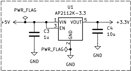
3.3 V MCU rail
