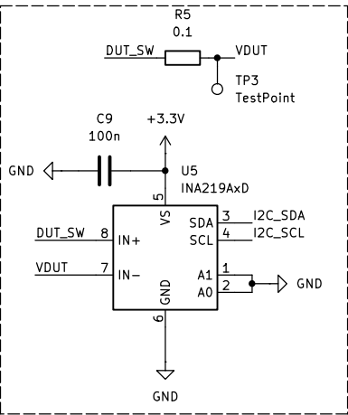
Current sense
