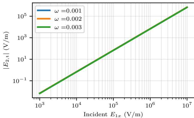
|E_{2,t}| vs incident E_{1x}
