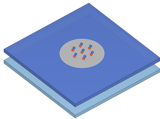
b) twisted bilayer graphene
