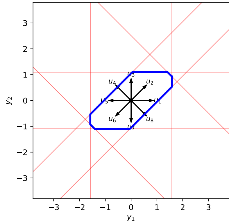
|U| = 8 directions
