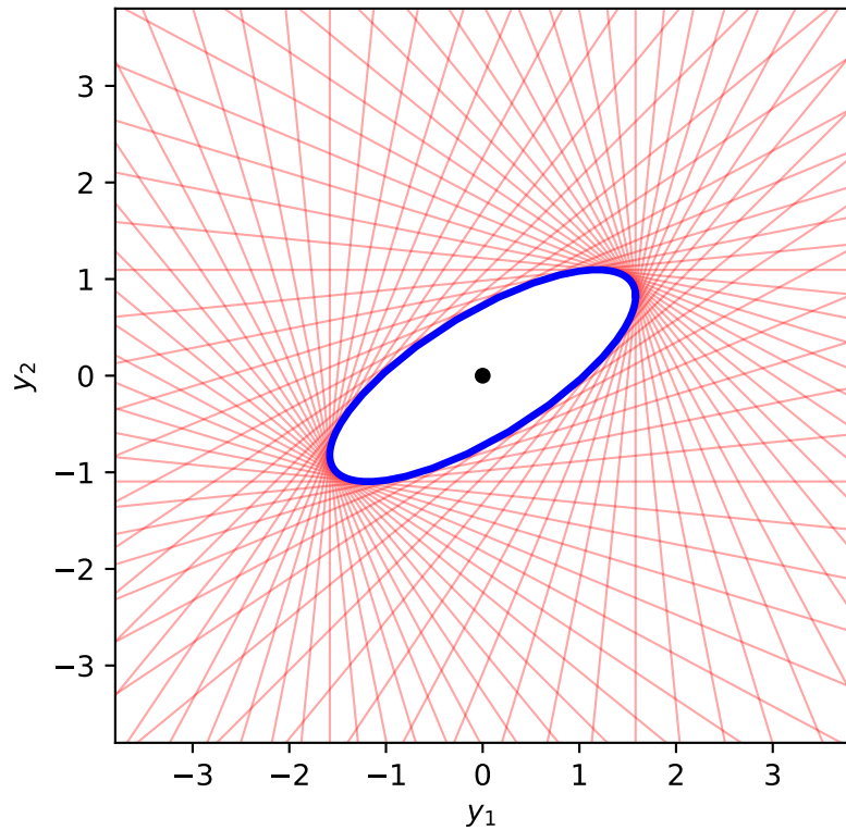
|U| = 64 directions
