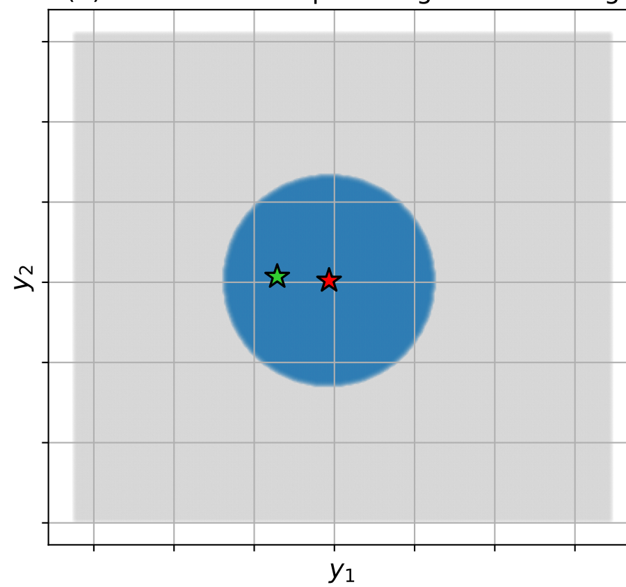
(b) MahalanobisEllipticalRegionNoLearning
