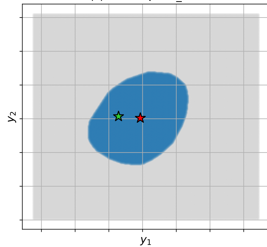
(c) VanillaQRNN_128
