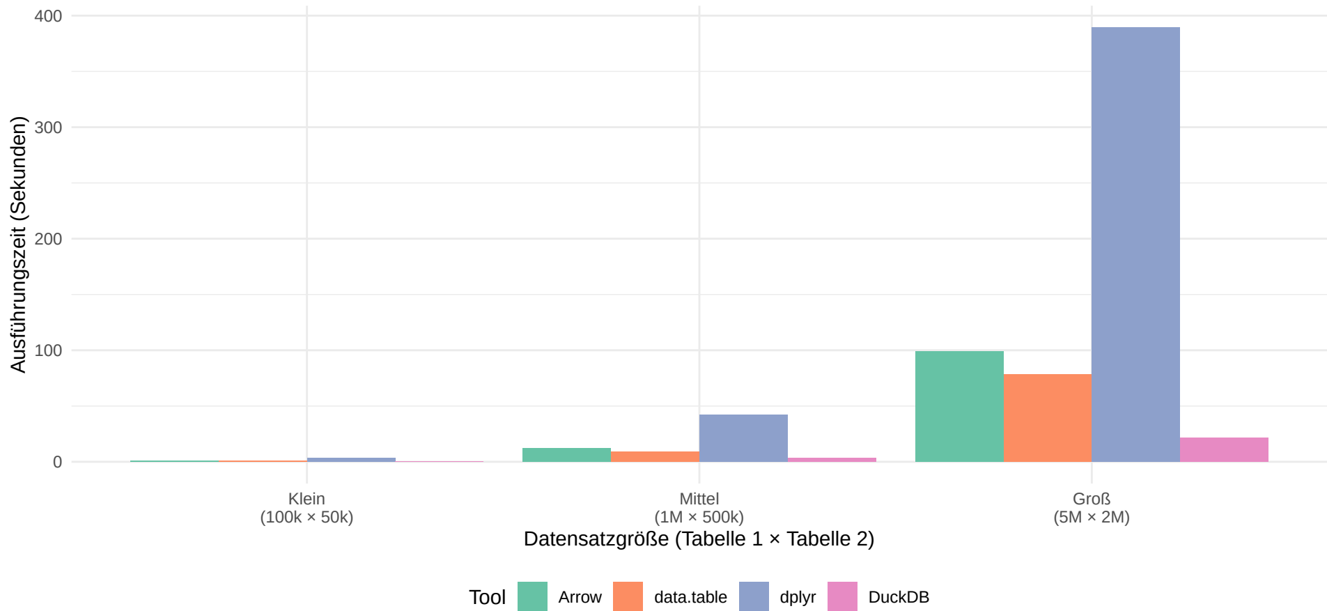
Join-Performance verschiedener Tools
