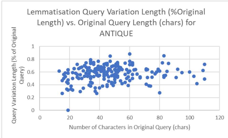
Figure 15; Perturbed queries are all either equal or shorter in length to original queries. For ANTIQUE dataset
