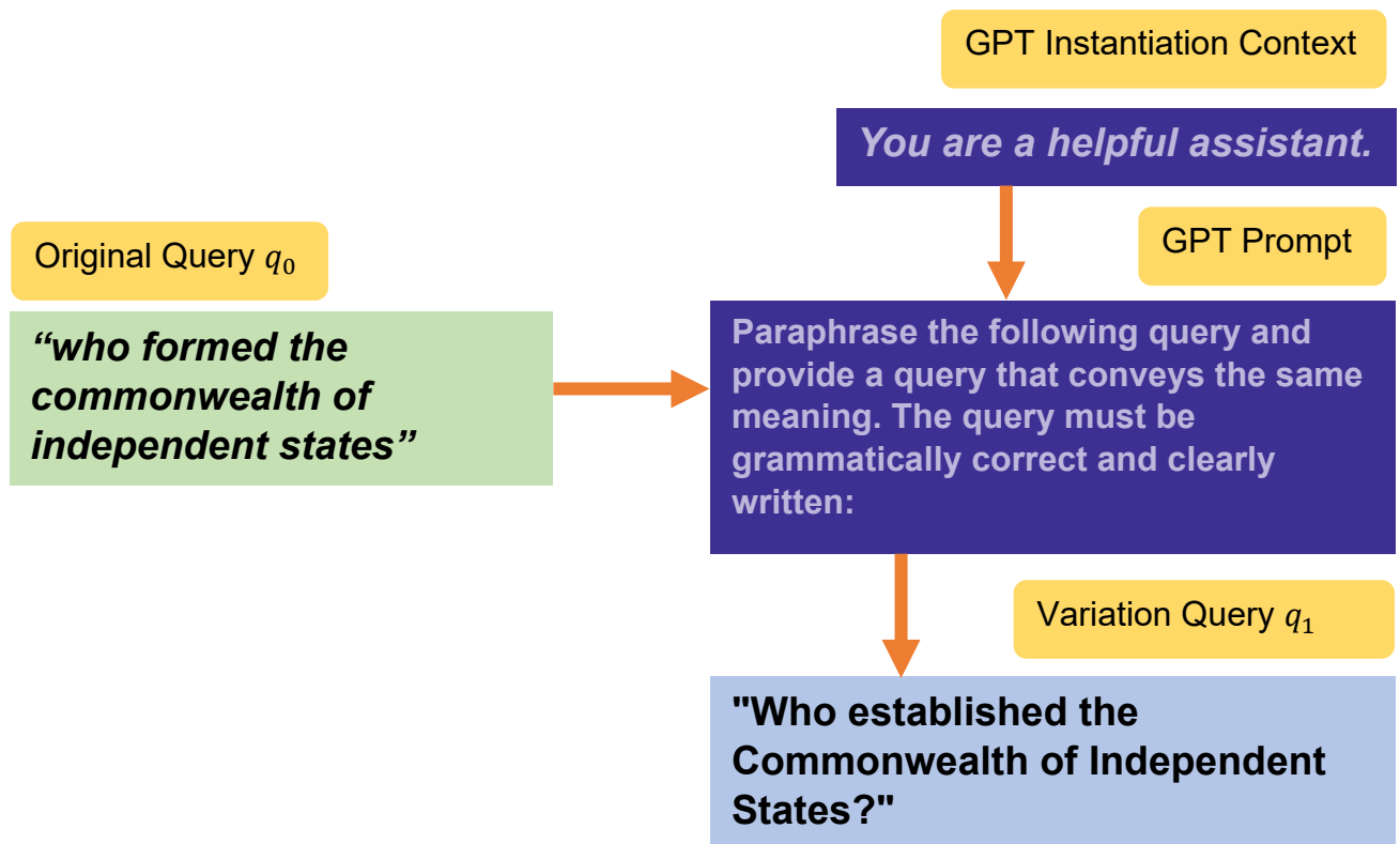
Figure 8; Process flow for generating a query variation using OpenAI GPT API
