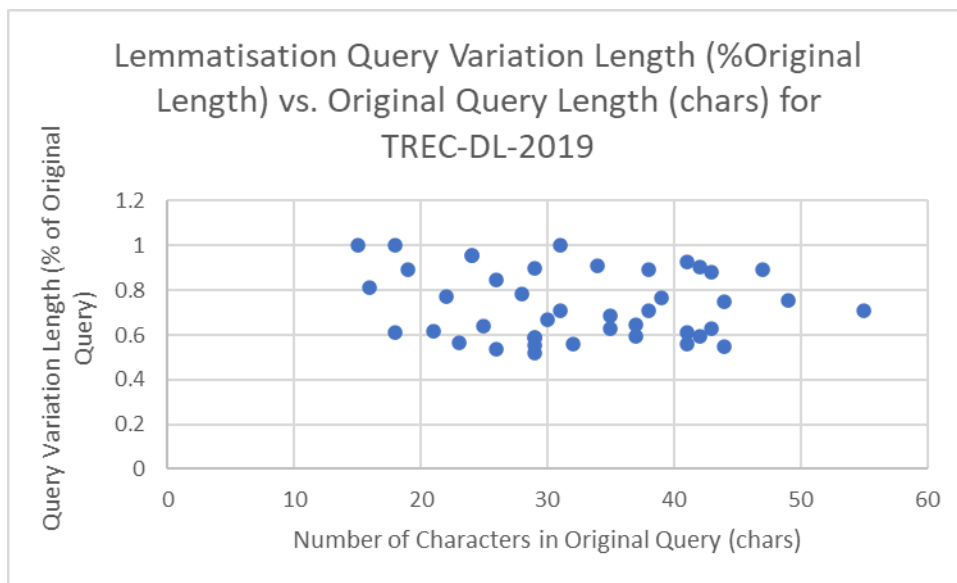
Figure 14; Increase in query variation length as a function of original query length (reported as a percentage). Perturbed queries are all either equal or shorter in length to original queries. For TREC-DL-2019 dataset
