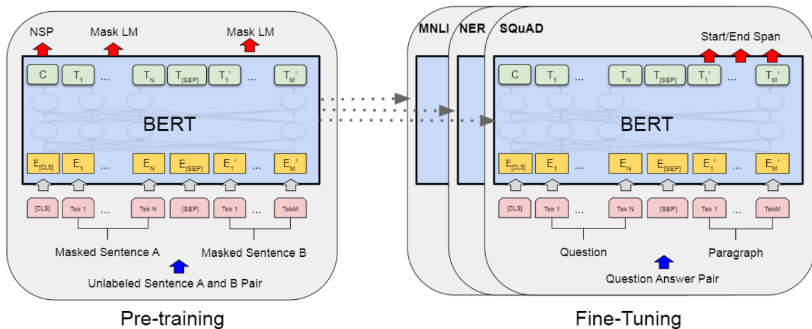
Figure 4; Excluding the output strata, identical architectural frameworks are employed throughout both pre-training and fine-tuning stages. Pre-trained model parameters are uniformly adopted as initial conditions across diverse downstream applications. Subsequent fine-tuning is applied to all parameters. The '[CLS]' token denotes a unique initiator symbol preceding each input instance, while '[SEP]' functions as a distinctive delimiter token, for instance, bifurcating questions and answers. From “BERT: Pre-training of Deep Bidirectional Transformers for Language Understanding” (pg. 3) by Devlin et al. 2018 [17]
