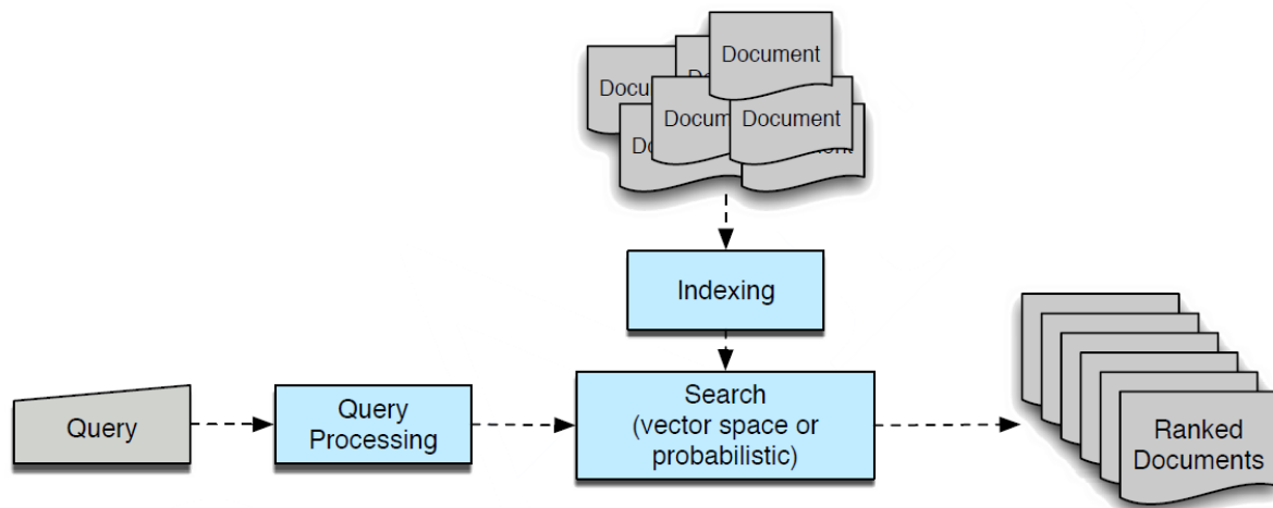
Figure 1; Simple representation of typical architecture of an ad-hoc retrieval system. Image Source: Jurafsky and Martin 2009 pg.782 [55]
