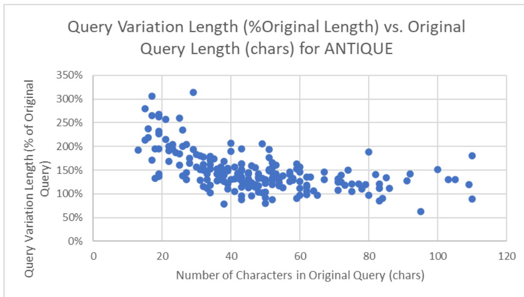
Figure 12; Increase in query variation length as a function of original query length (reported as a percentage). Shorter queries are more often represented by longer generated queries. For ANTIQUE dataset
