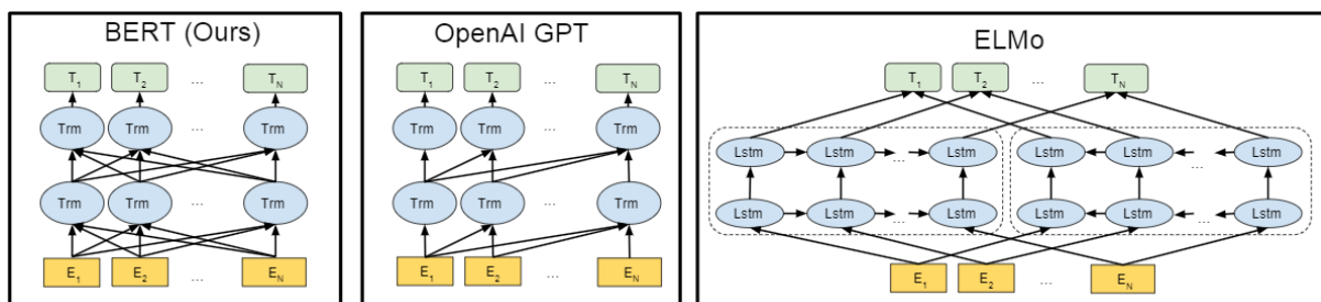
Figure 5; BERT employs a bidirectional Transformer, conditioning on both left and right contexts across all layers. GPT uses a left-to-right Transformer, predicting each token based on its predecessors. ELMo utilizes bidirectional LSTMs, generating features from both directions independently. BERT and GPT are fine-tuned, adapting pre-trained models to specific tasks, whereas ELMo provides features for task-specific model enhancement. From
