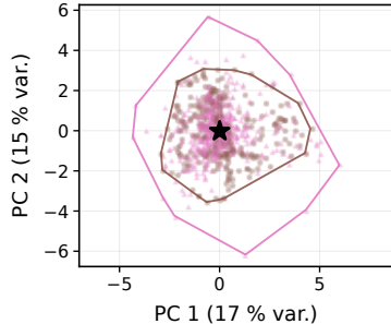
PCA of standardised \dot{q} only, 12-D
