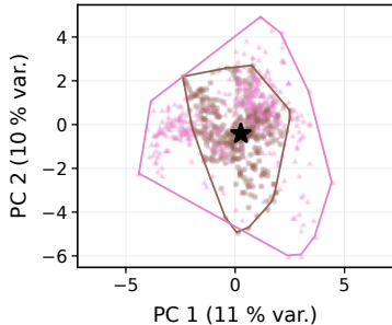
PCA of standardised (q, \dot{q}) , 24-D
