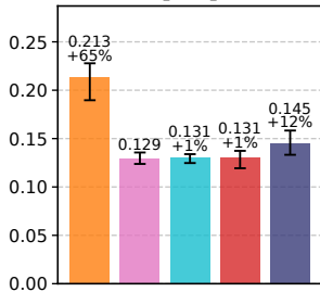
Tracking Error Yaw [rad]
