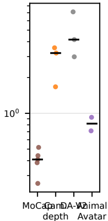
M2 jitter by source [% of L]
