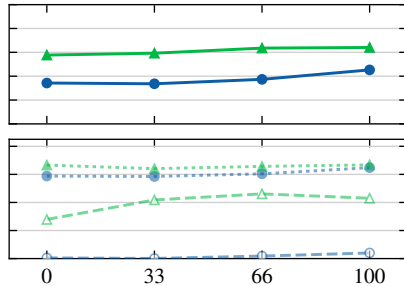
(b) % of LIBERO-90 as play data
