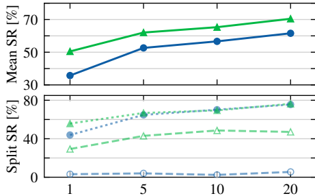
(a) # Episodes with action labels
