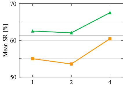
(c) # X-embodiments in video pretraining
