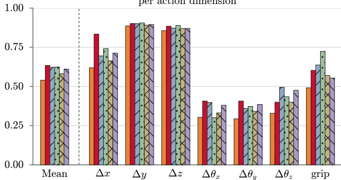
MLP R^2 , mean over benchmarks
