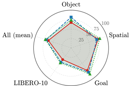
Non-Held-Out Tasks
