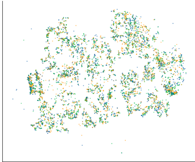
70k steps
