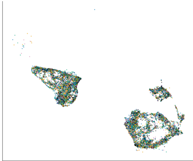
70k steps
