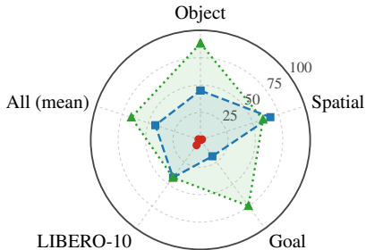
Held-Out Tasks
