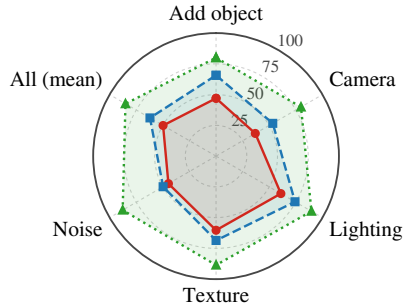
LIBERO-Plus Disturbances
