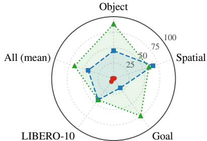
Held-Out Tasks
