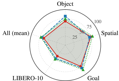
Non-Held-Out Tasks
