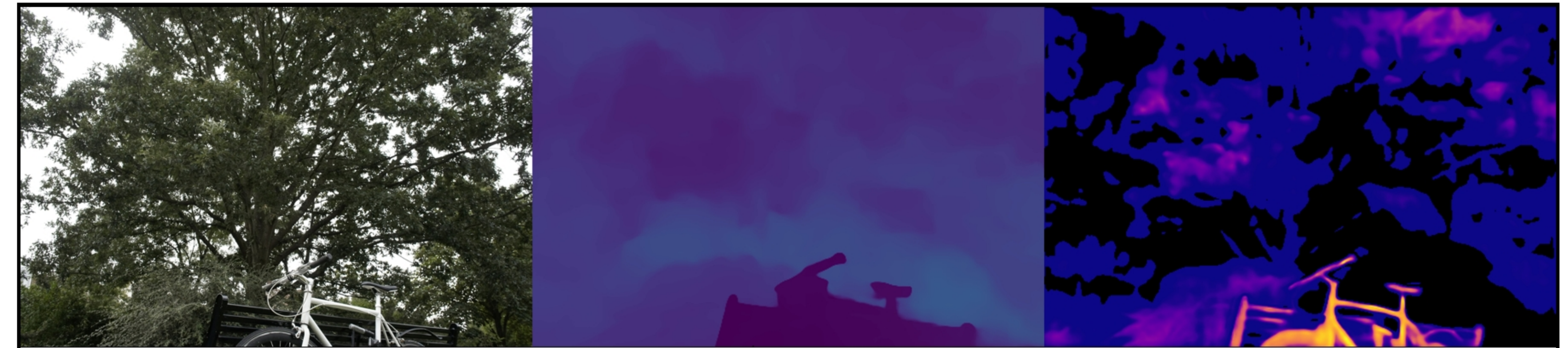
bicycle: VGGT | num_images=20 Original | Depth (max=2.81) | Confidence (max=3.28)
