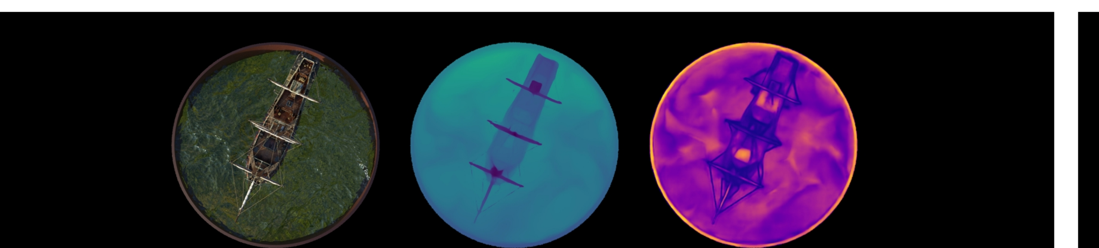
ship: VGGT | num_images=30 Original | Depth (max=1.06) | Confidence (max=129.55)
