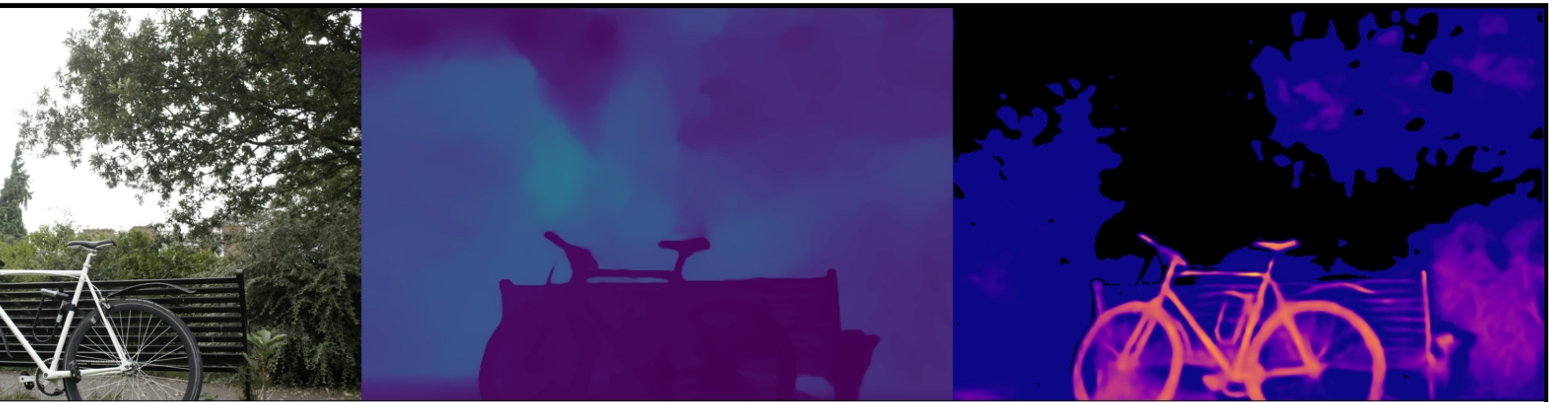
bicycle: VGGT | num_images=100 Original | Depth (max=2.93) | Confidence (max=3.80)
