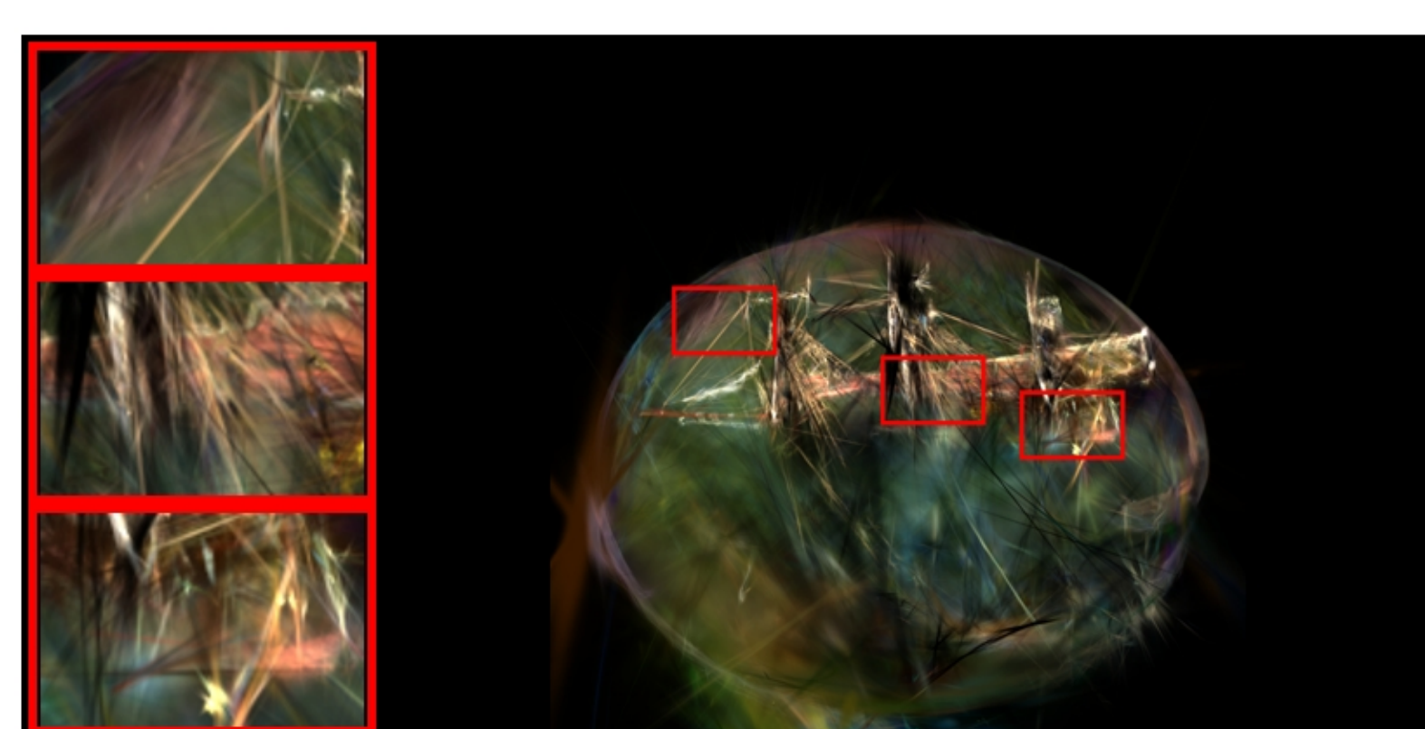
ship: COLMAP | num_images=30 PSNR: 16.89 | LPIPS: 0.4083 | SSIM: 0.5997
