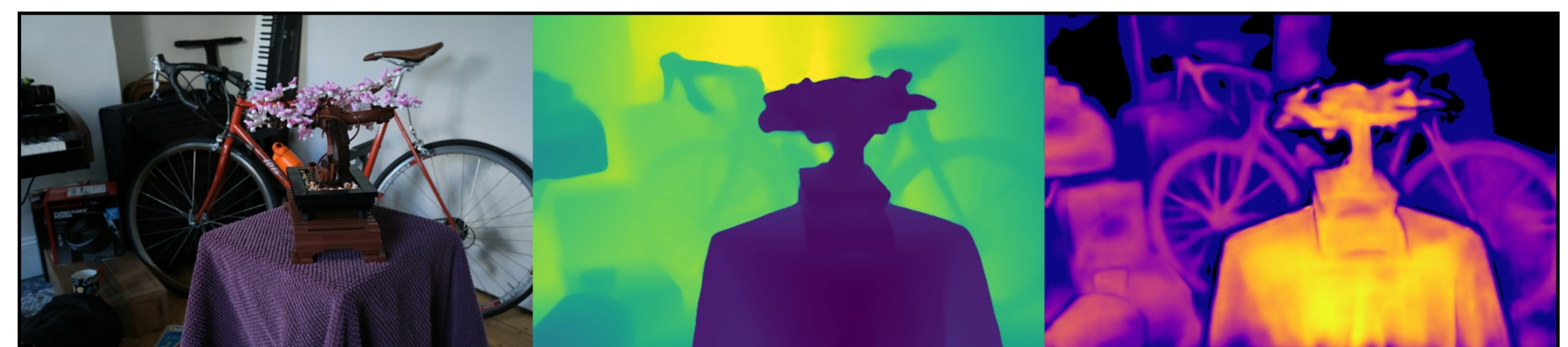
bonsai: VGGT | num_images=40 Original | Depth (max=2.20) | Confidence (max=4.74)
