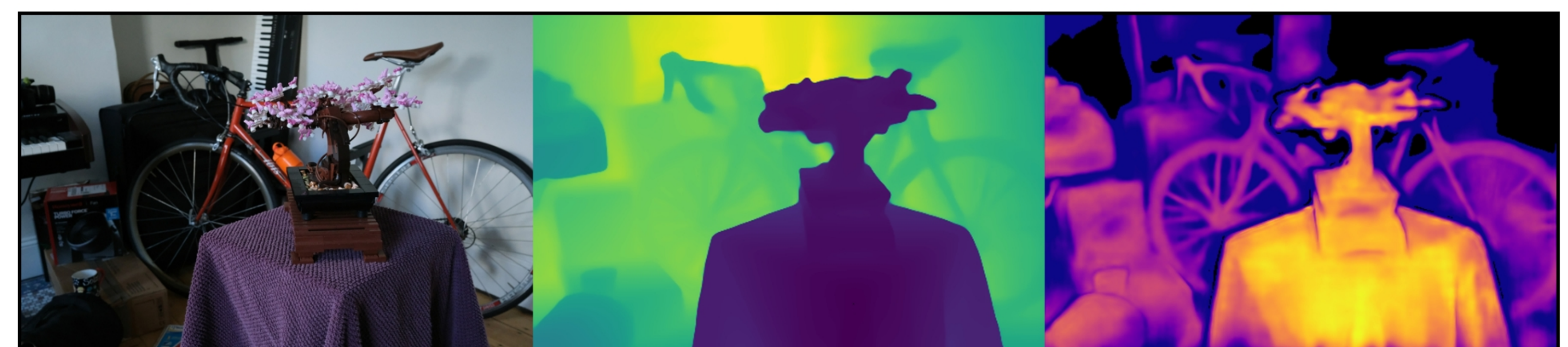
bonsai: VGGT | num_images=100 Original | Depth (max=2.16) | Confidence (max=5.62)
