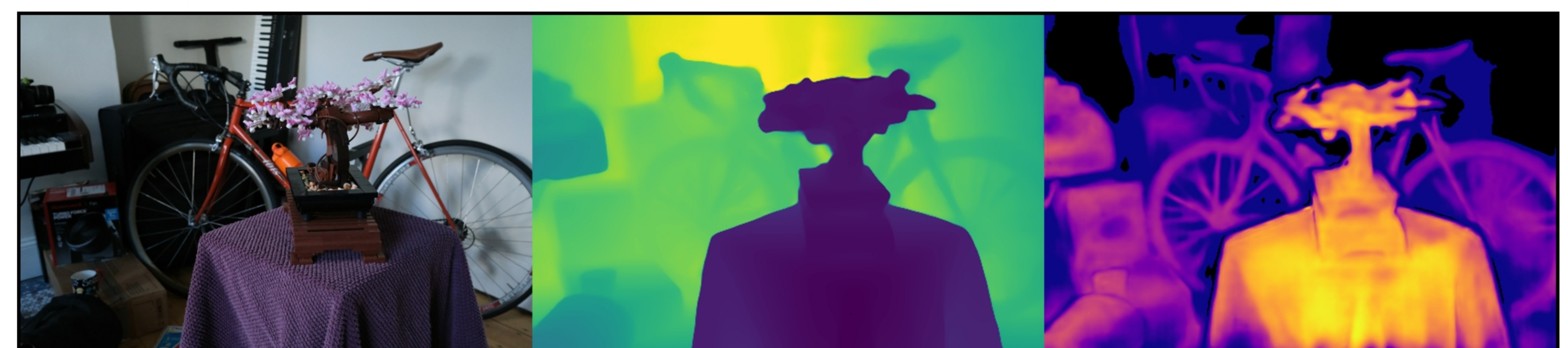
bonsai: VGGT | num_images=20 Original | Depth (max=2.24) | Confidence (max=4.36)
