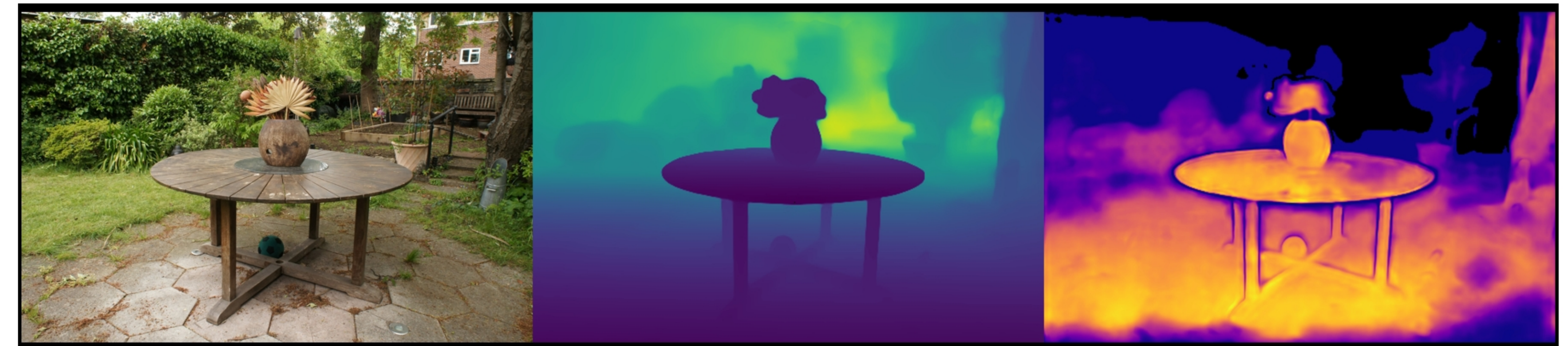
garden: VGGT | num_images=30 Original | Depth (max=2.72) | Confidence (max=7.15)
