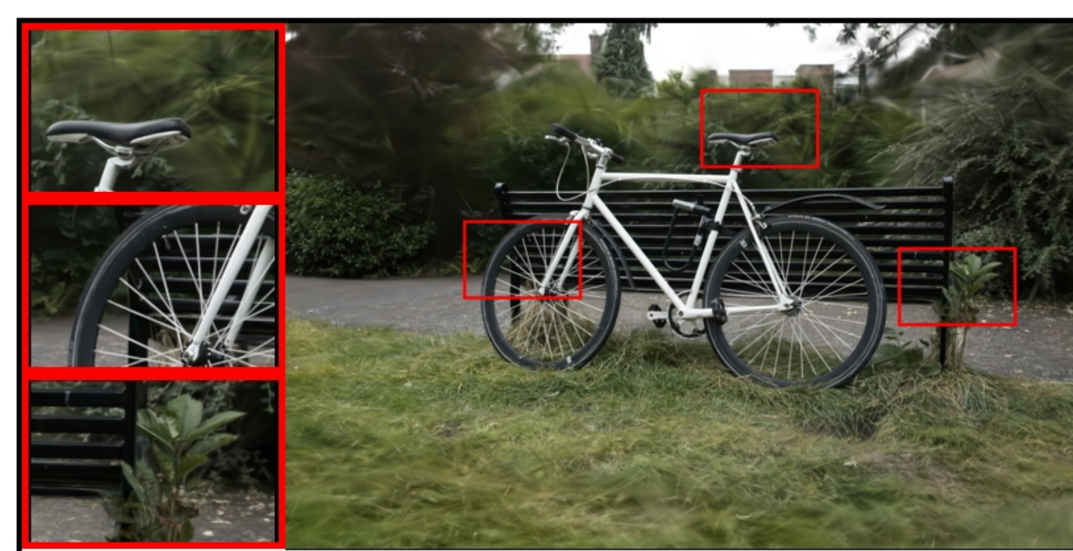
bicycle: COLMAP | num_images=100 PSNR: 21.35 | LPIPS: 0.3071 | SSIM: 0.4816
