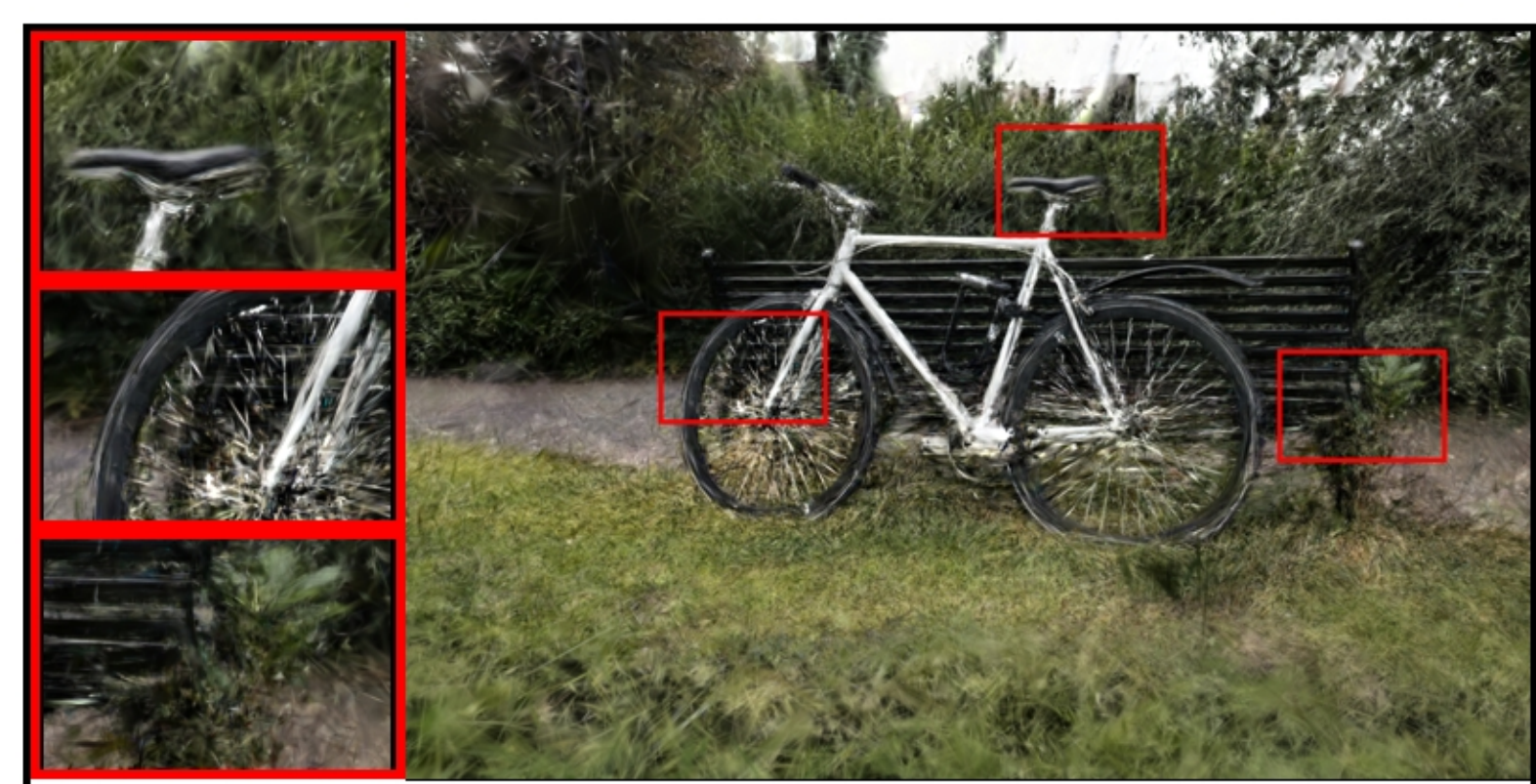
bicycle: VGGT | num_images=30 PSNR: 16.64 | LPIPS: 0.4168 | SSIM: 0.2121
