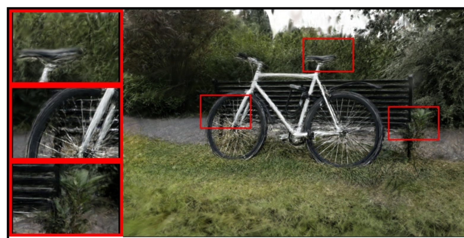
bicycle: VGGT | num_images=70 PSNR: 17.30 | LPIPS: 0.4162 | SSIM: 0.2482
