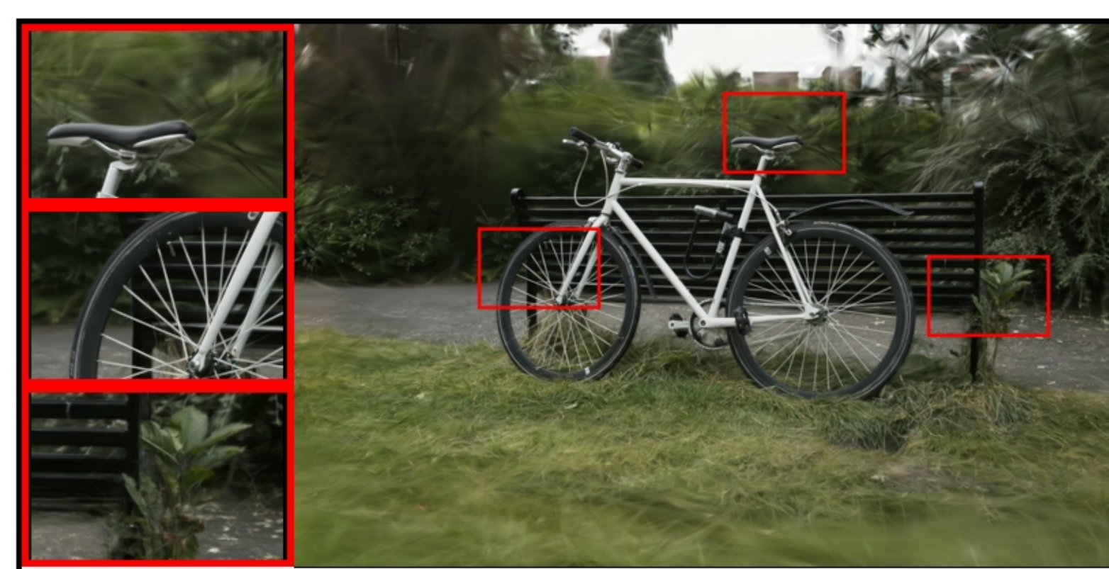
bicycle: COLMAP | num_images=70 PSNR: 19.71 | LPIPS: 0.3646 | SSIM: 0.3701
