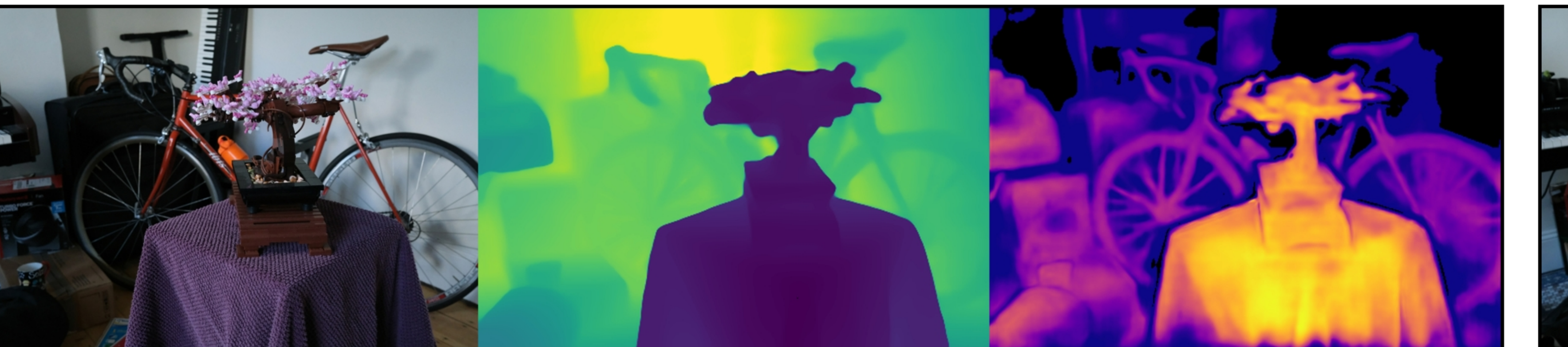
bonsai: VGGT | Pose Opt | num_images=30 Original | Depth (max=2.25) | Confidence (max=4.34)
