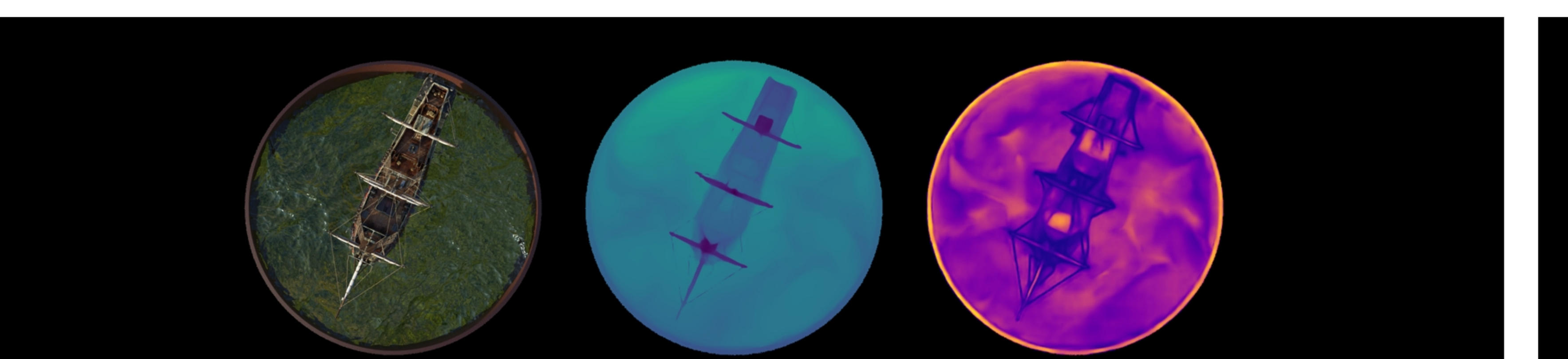
ship: VGGT | Pose Opt | num_images=30 Original | Depth (max=1.06) | Confidence (max=129.55)
