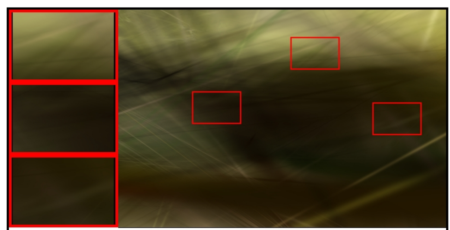
bicycle: COLMAP | Pose Opt | num_images=30 PSNR: 12.71 | LPIPS: 0.8428 | SSIM: 0.2465
