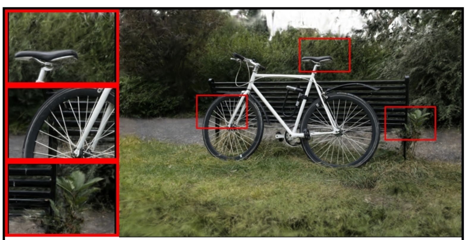
bicycle: VGGT | Pose Opt | num_images=70 PSNR: 17.14 | LPIPS: 0.3577 | SSIM: 0.2516
