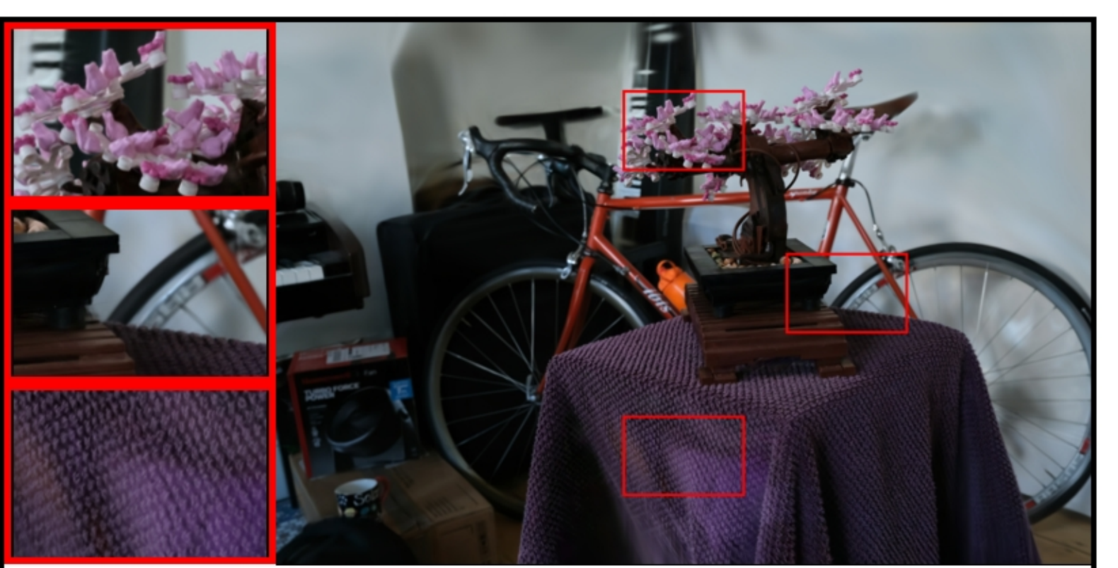
bonsai: COLMAP | Pose Opt | num_images=100 PSNR: 25.54 | LPIPS: 0.1440 | SSIM: 0.7955
