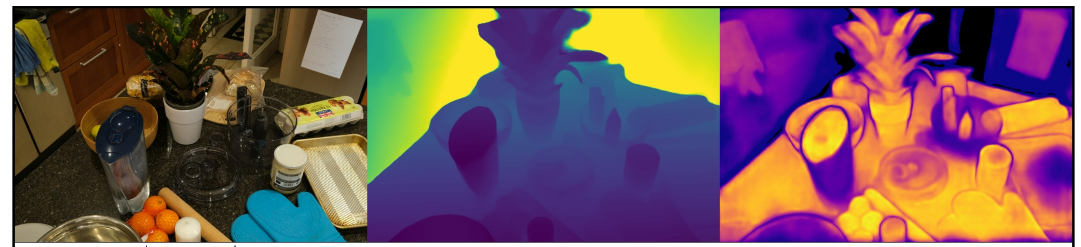
counter: VGGT | Pose Opt | num_images=30 Original | Depth (max=2.48) | Confidence (max=13.28)
