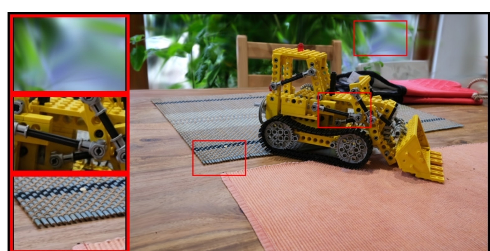
kitchen: COLMAP | Pose Opt | num_images=100 PSNR: 22.44 | LPIPS: 0.1272 | SSIM: 0.5514
