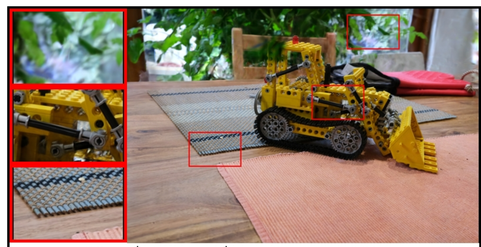
kitchen: VGGT | Pose Opt | num_images=30 PSNR: 19.22 | LPIPS: 0.2184 | SSIM: 0.4837
