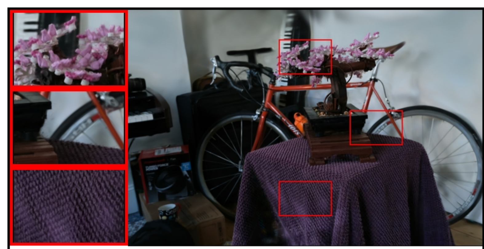
bonsai: VGGT | Pose Opt | num_images=100 PSNR: 18.46 | LPIPS: 0.3355 | SSIM: 0.5824
