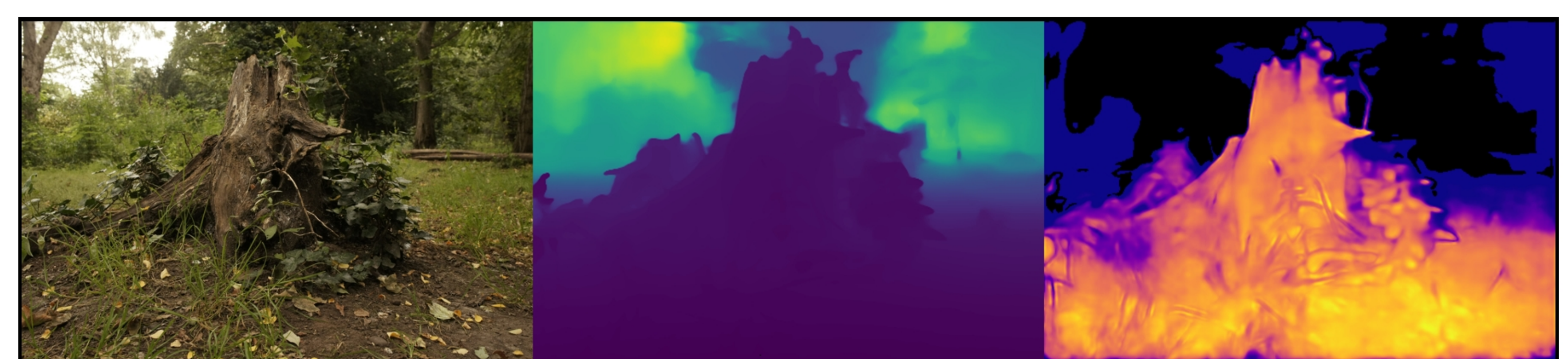
stump: VGGT | Pose Opt | num_images=70 Original | Depth (max=6.33) | Confidence (max=2.42)
