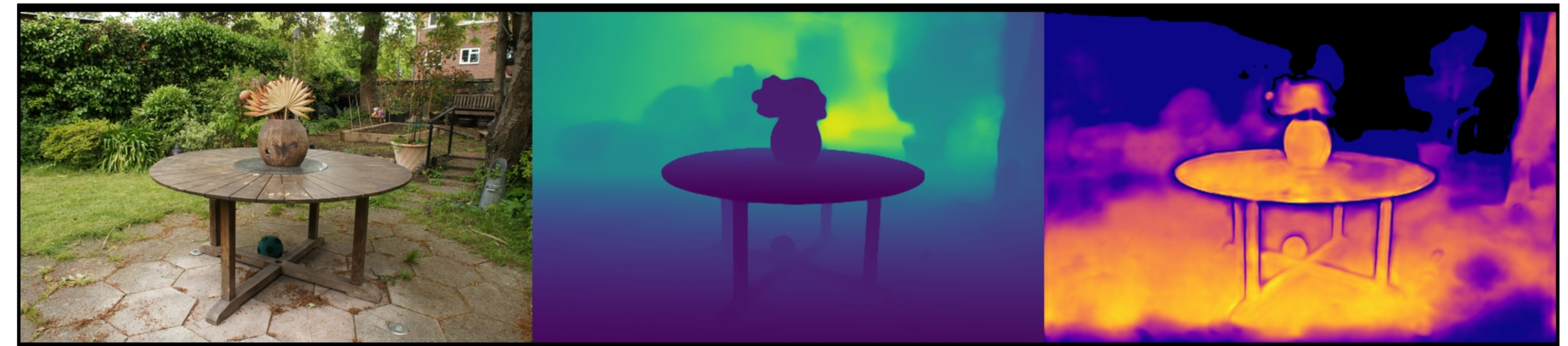
garden: VGGT | Pose Opt | num_images=20 Original | Depth (max=2.75) | Confidence (max=6.97)
