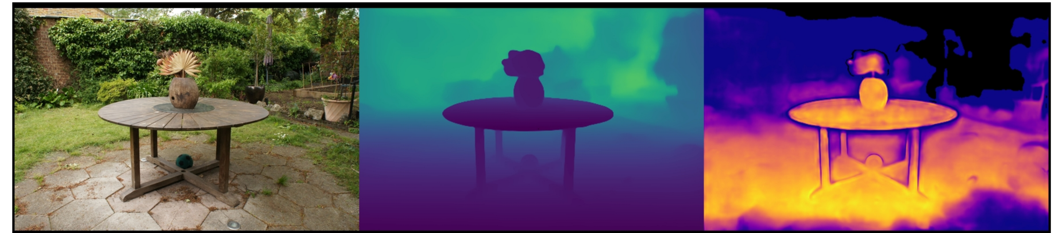
garden: VGGT | Pose Opt | num_images=70 Original | Depth (max=2.46) | Confidence (max=6.77)
