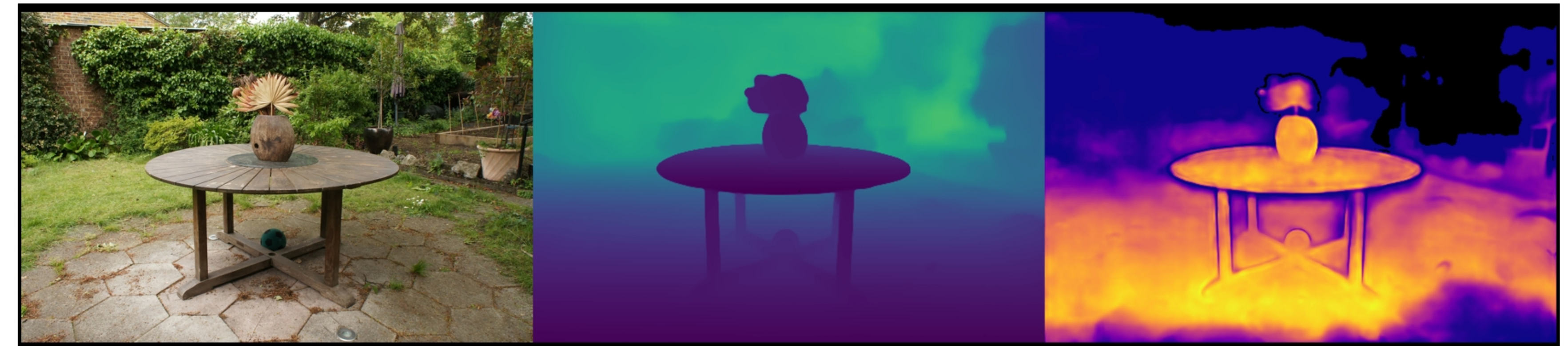
garden: VGGT | Pose Opt | num_images=100 Original | Depth (max=2.46) | Confidence (max=7.08)
