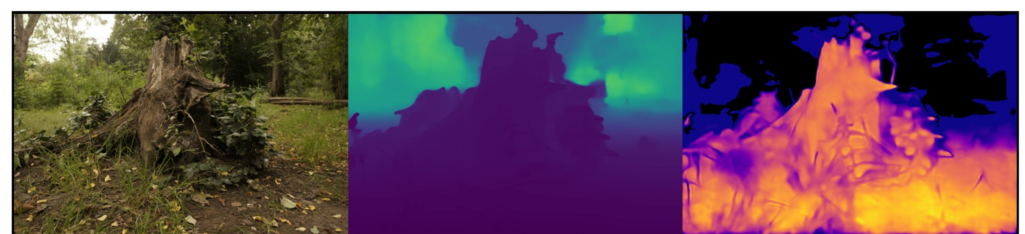
stump: VGGT | Pose Opt | num_images=30 Original | Depth (max=5.75) | Confidence (max=4.28)
