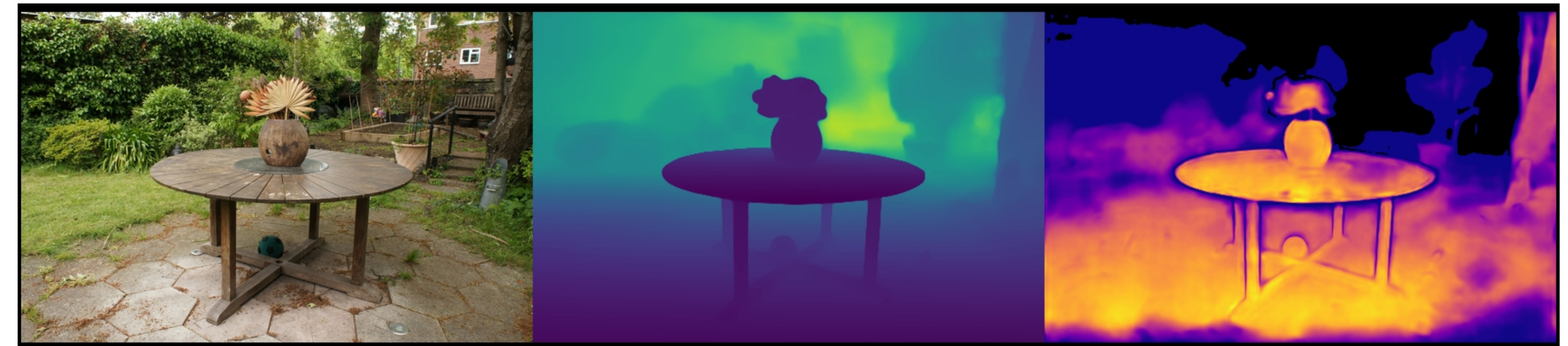
garden: VGGT | Pose Opt | num_images=40 Original | Depth (max=2.72) | Confidence (max=7.67)
