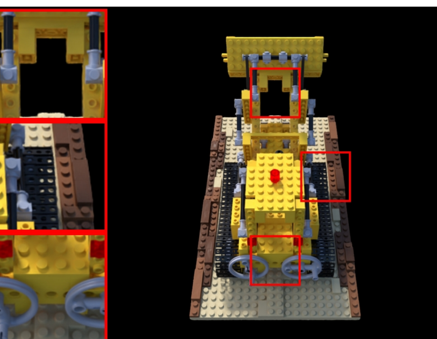
lego: VGGT | Pose Opt | num_images=87 PSNR: 20.35 | LPIPS: 0.0759 | SSIM: 0.7735
