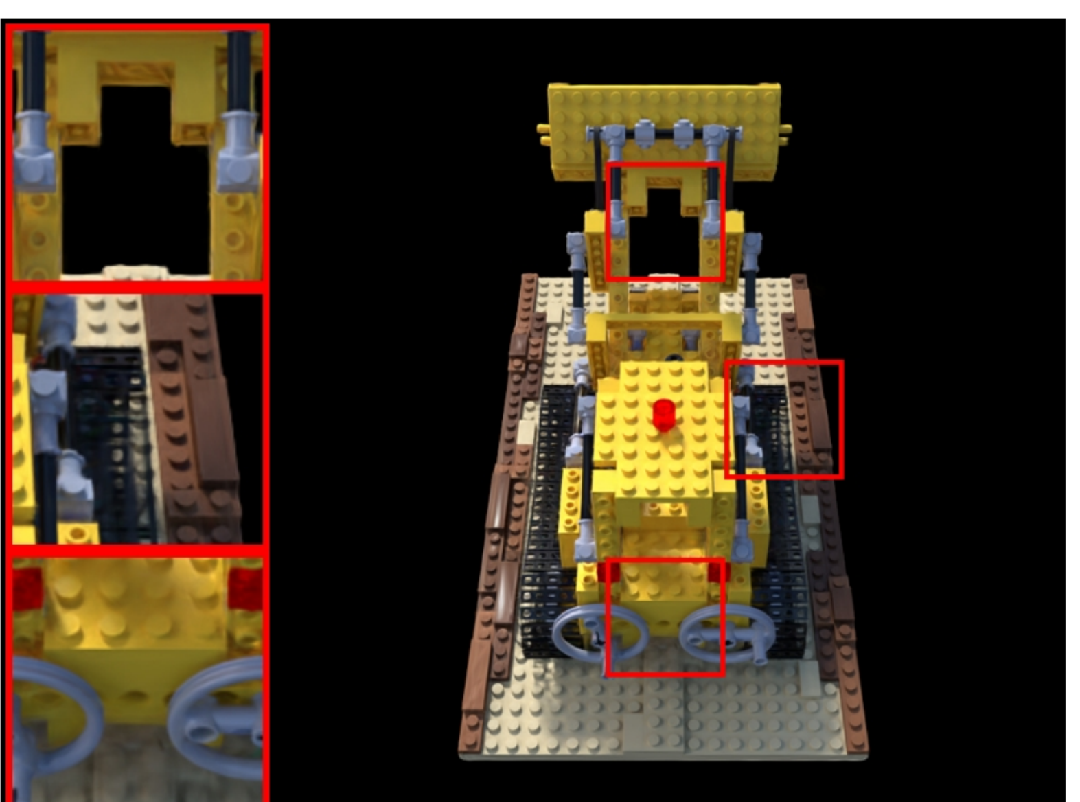
lego: COLMAP | Pose Opt | num_images=40 PSNR: 20.58 | LPIPS: 0.0849 | SSIM: 0.8054
