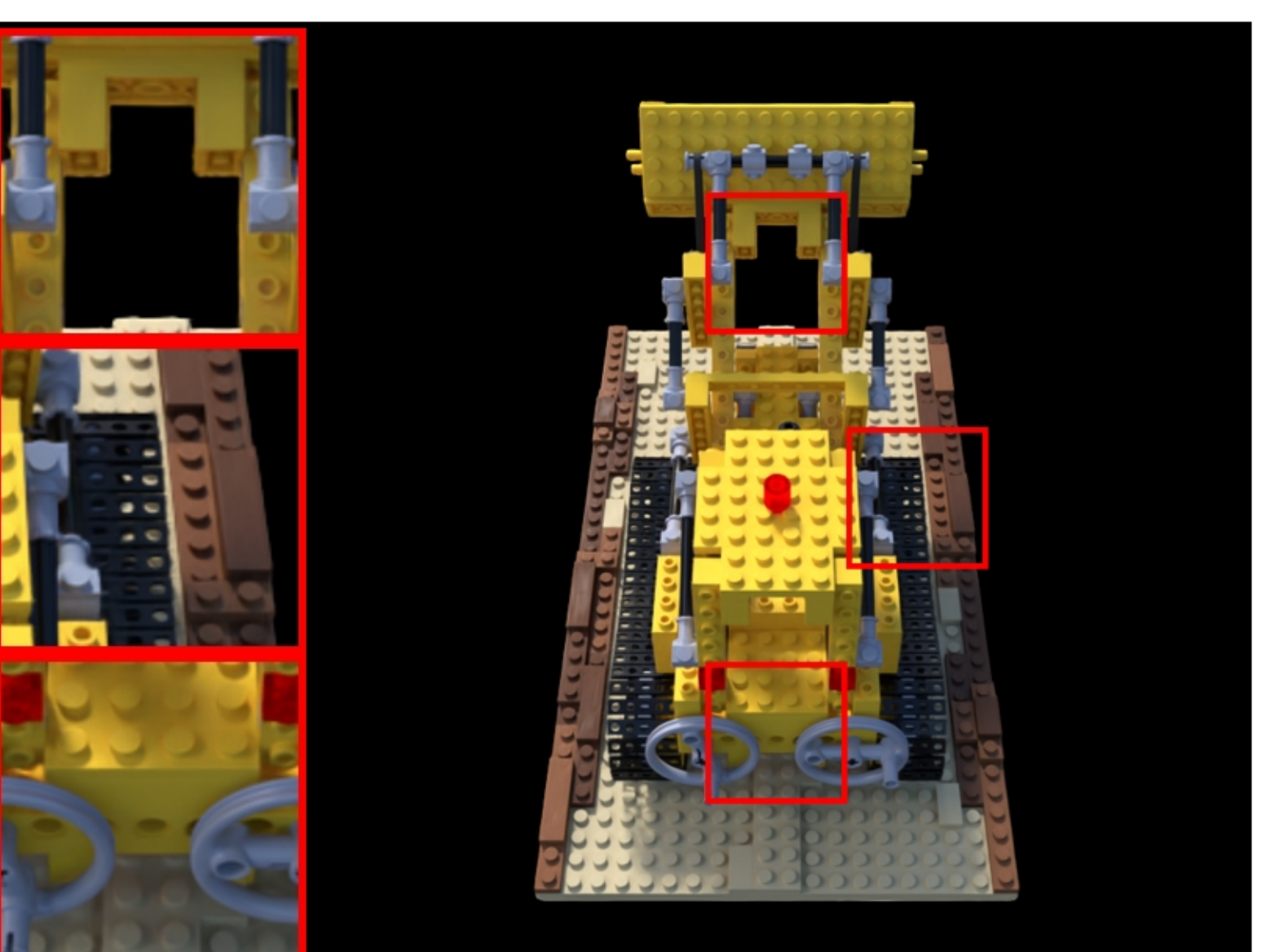
lego: COLMAP | Pose Opt | num_images=70 PSNR: 23.03 | LPIPS: 0.0640 | SSIM: 0.8601
