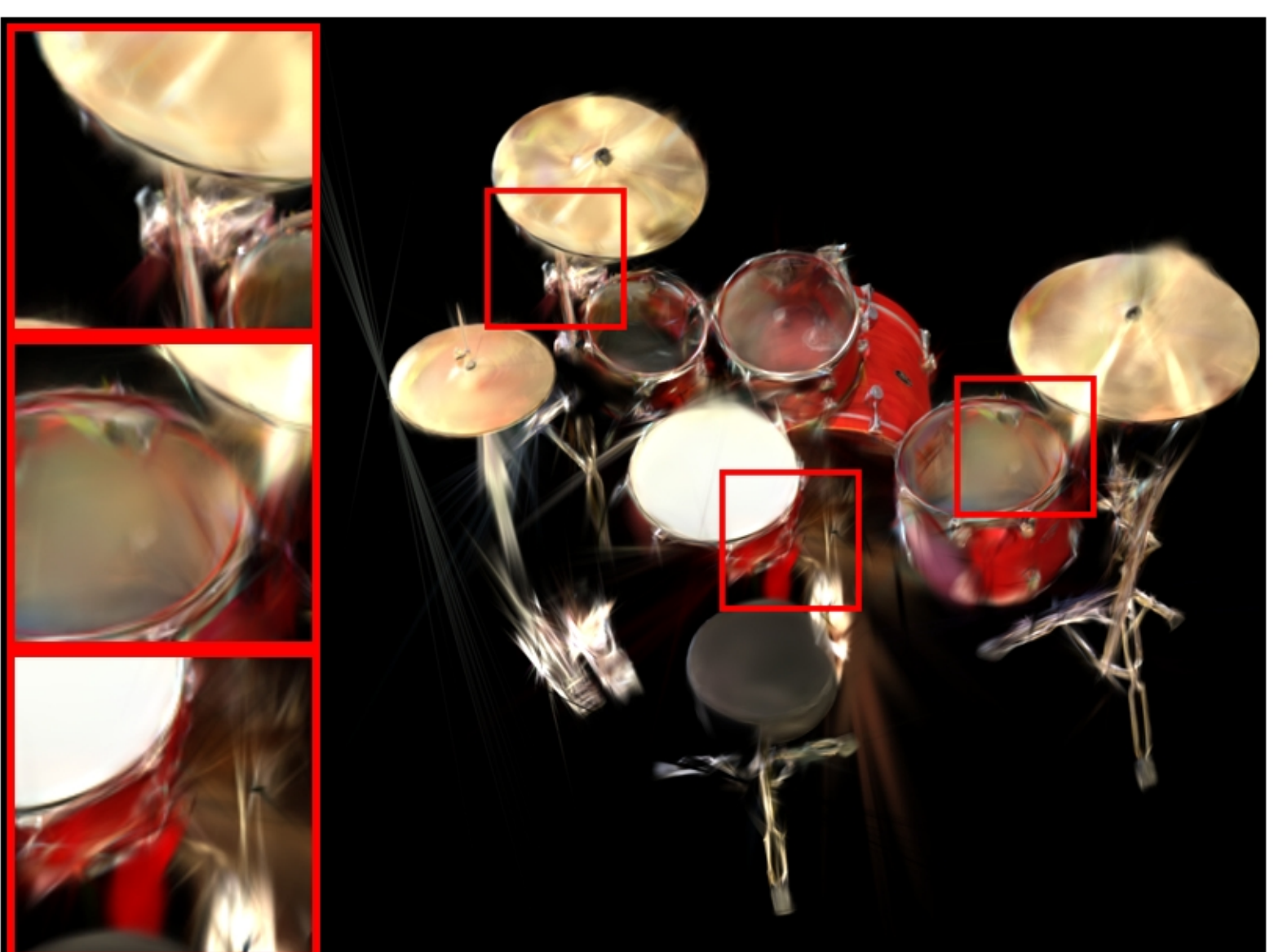
drums: COLMAP | Pose Opt | num_images=40 PSNR: 15.96 | LPIPS: 0.2388 | SSIM: 0.7241
