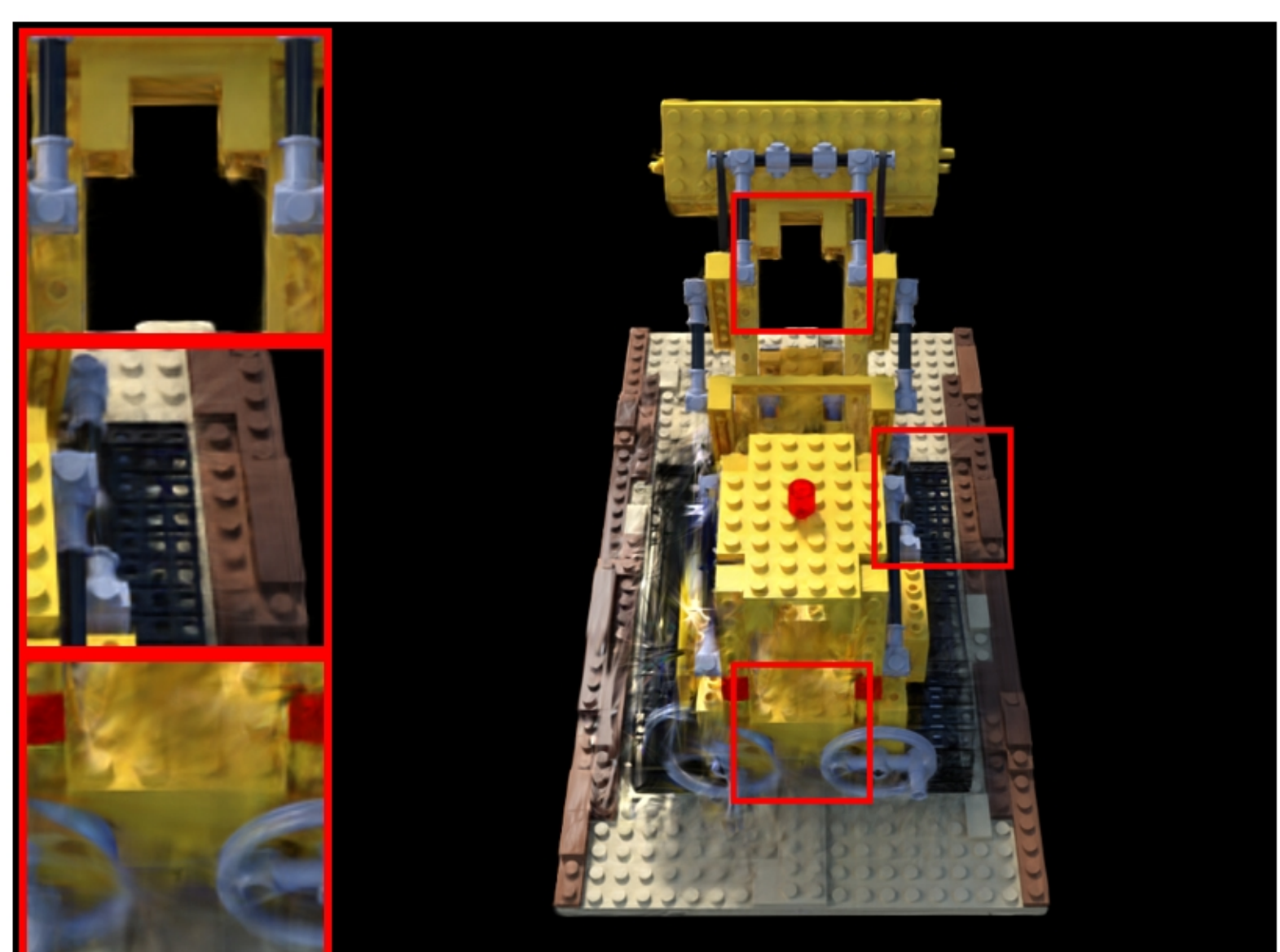
lego: COLMAP | Pose Opt | num_images=30 PSNR: 16.64 | LPIPS: 0.2402 | SSIM: 0.6695
