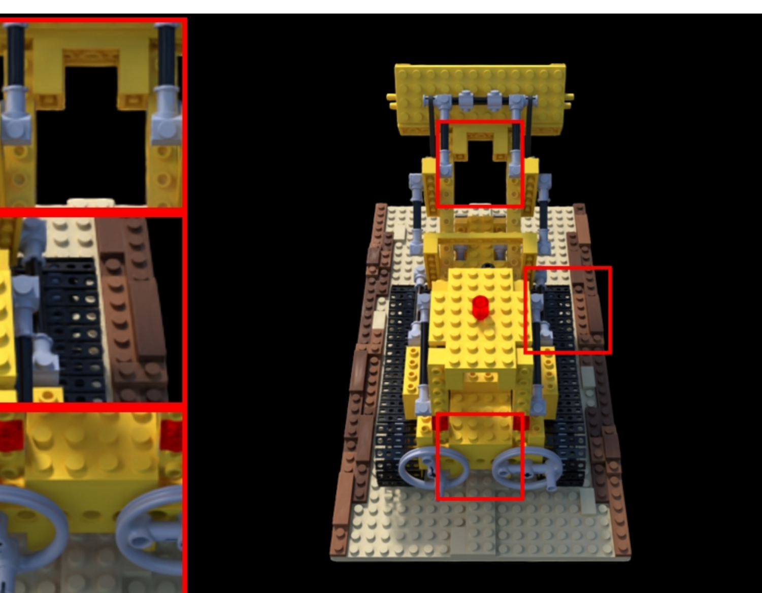
lego: COLMAP | Pose Opt | num_images=87 PSNR: 23.42 | LPIPS: 0.0607 | SSIM: 0.8655
