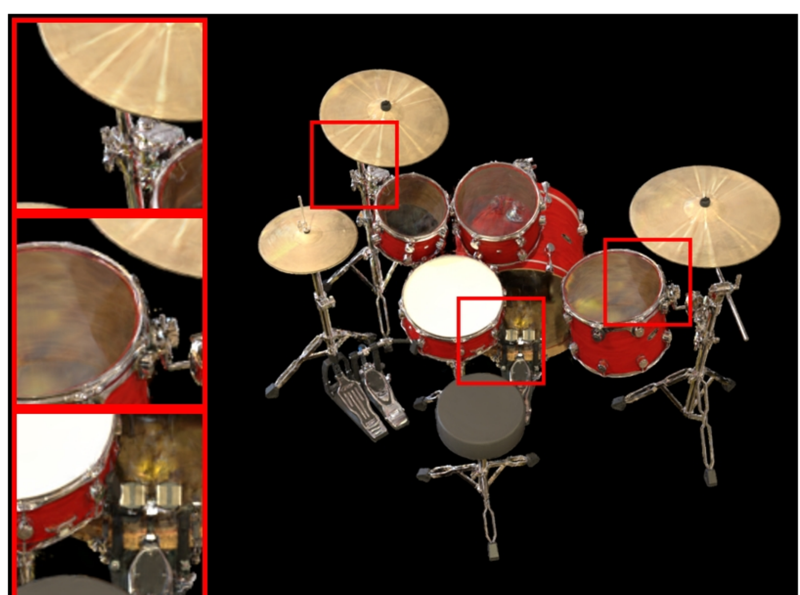
drums: VGGT | Pose Opt | num_images=30 PSNR: 19.73 | LPIPS: 0.0802 | SSIM: 0.8435
