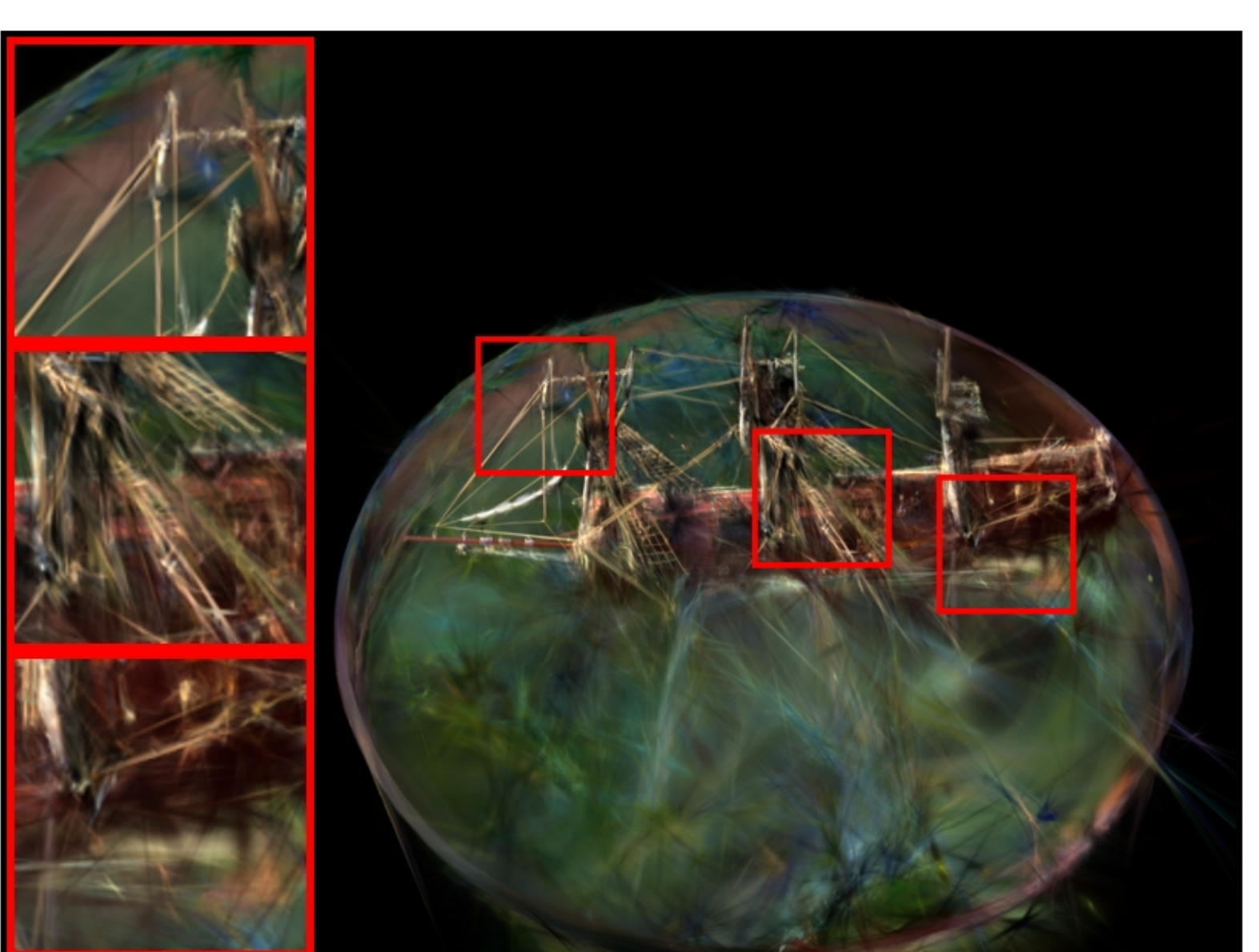
ship: COLMAP | Pose Opt | num_images=40 PSNR: 19.10 | LPIPS: 0.2918 | SSIM: 0.6571
