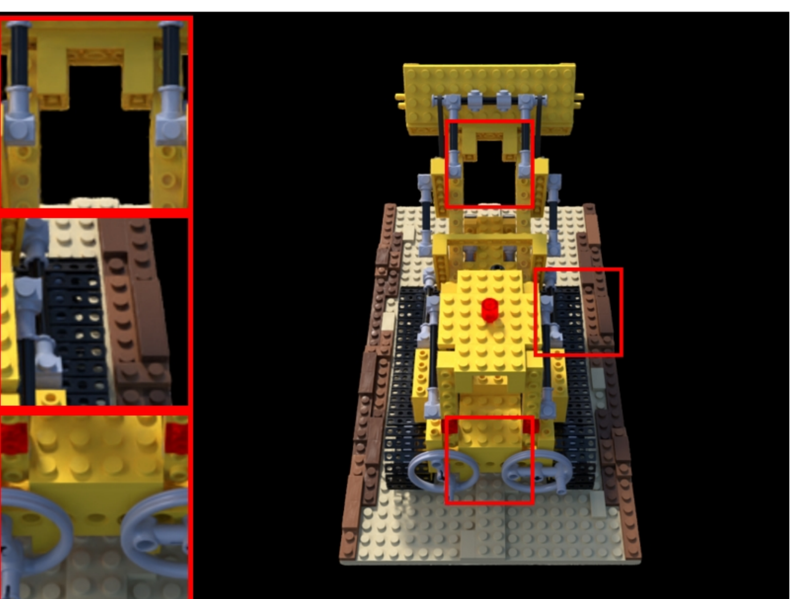
lego: VGGT | Pose Opt | num_images=70 PSNR: 19.62 | LPIPS: 0.0837 | SSIM: 0.7626
