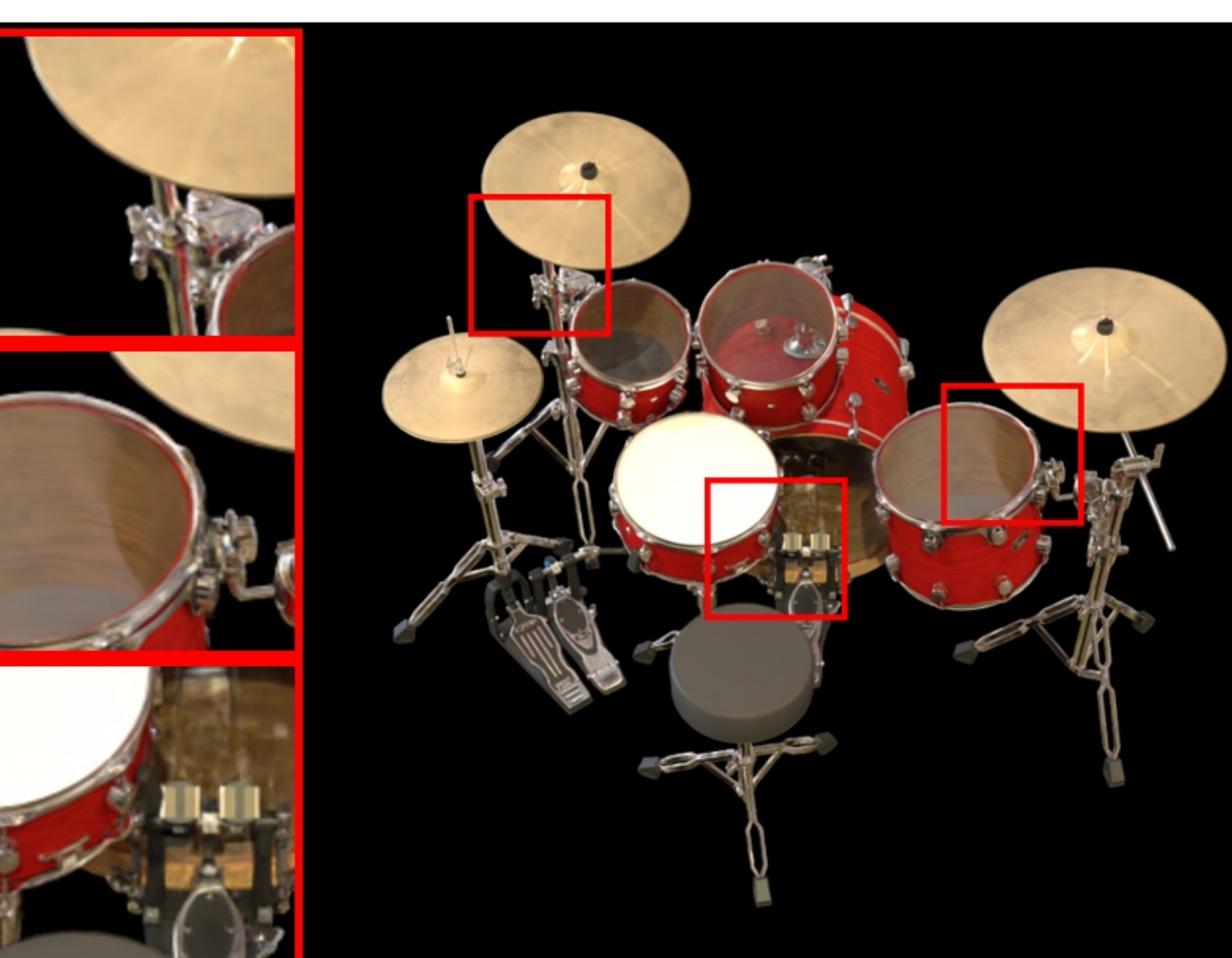
drums: VGGT | Pose Opt | num_images=87 PSNR: 20.90 | LPIPS: 0.0848 | SSIM: 0.8690
