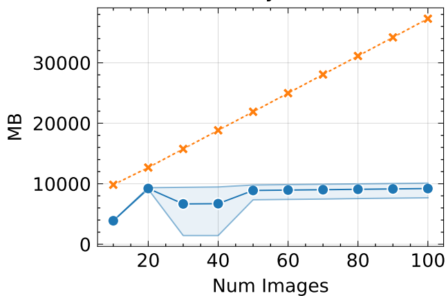
Peak Memory ↓ - outdoor
