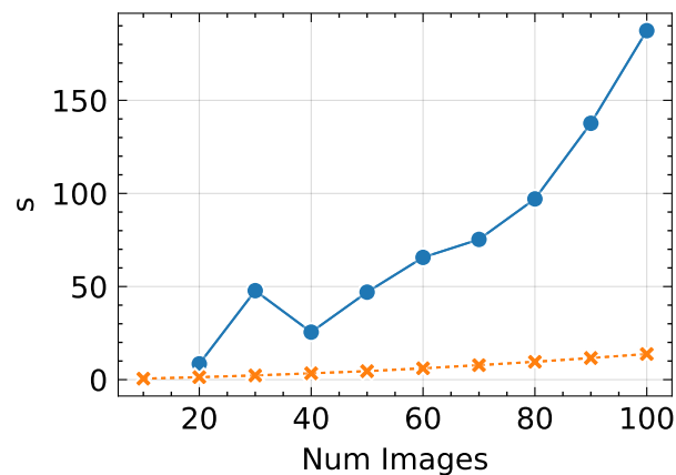
Inference Time ↓ - bonsai
