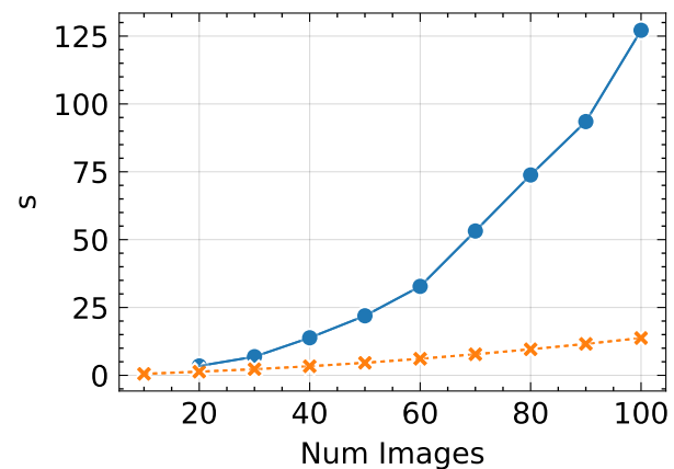
Inference Time ↓ - kitchen
