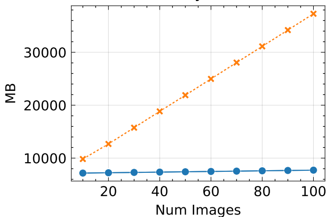
Peak Memory ↓ - counter
