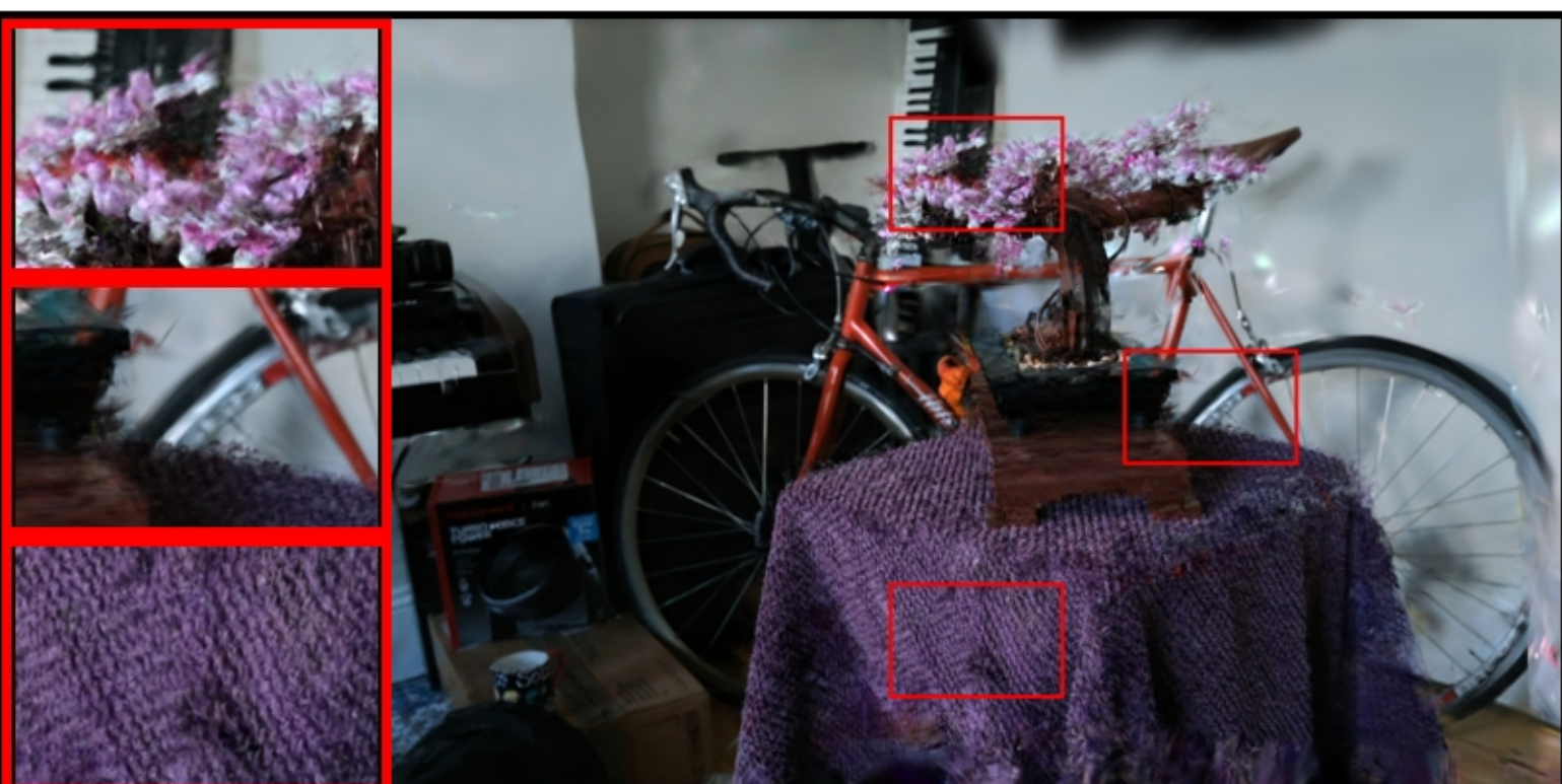
bonsai: VGGT | num_images=20 PSNR: 16.74 | LPIPS: 0.4367 | SSIM: 0.5235
