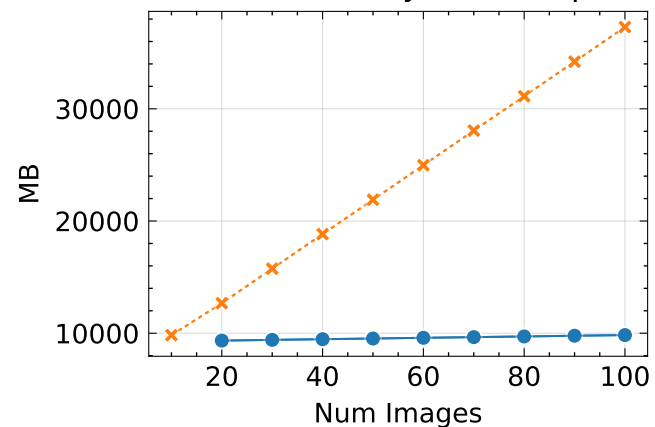
Peak Memory ↓ - stump
