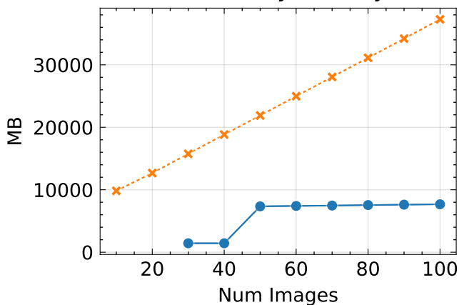
Peak Memory ↓ - bicycle
