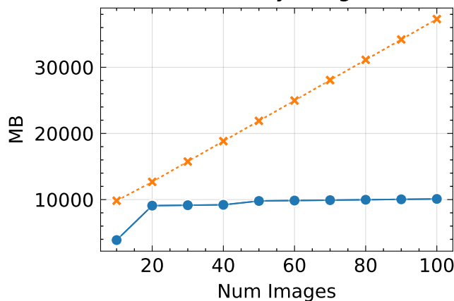
Peak Memory ↓ - garden
