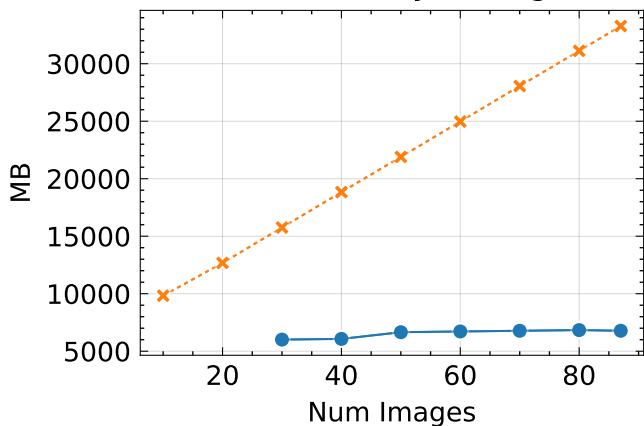
Peak Memory ↓ - lego
