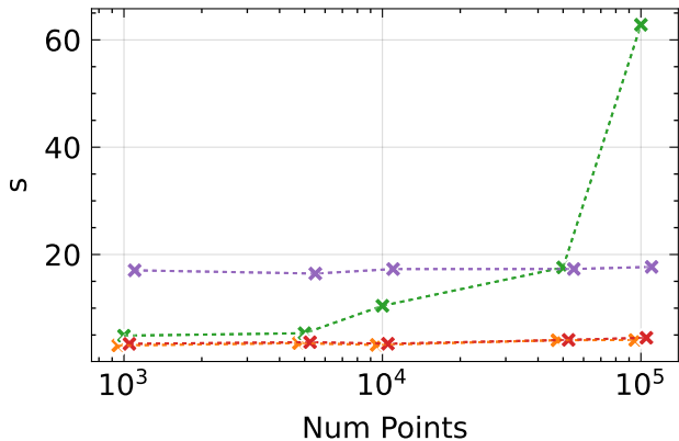
Pcd Processing Time ↓ - bonsai
