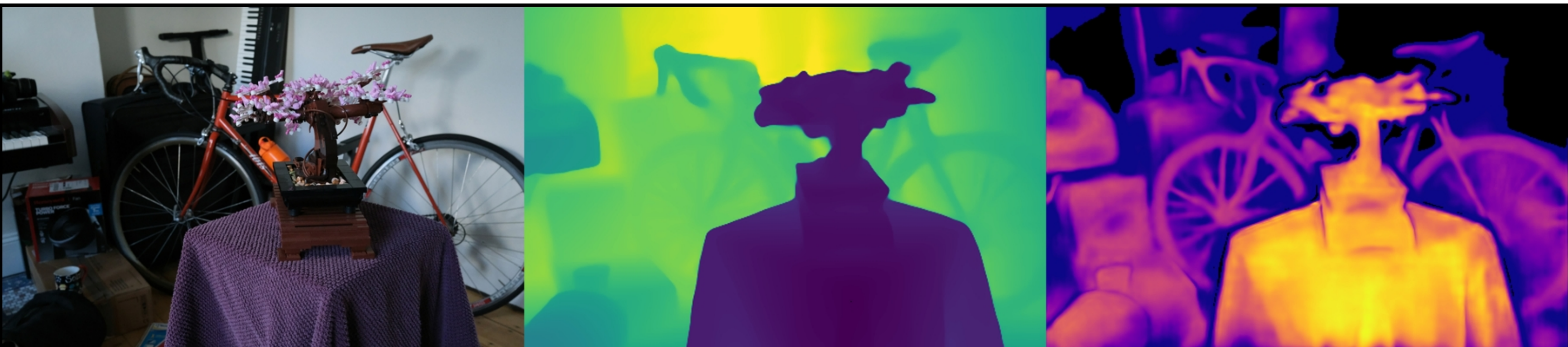
bonsai: VGGT | ba | num_points=23313 Original | Depth (max=2.16) | Confidence (max=5.62)
