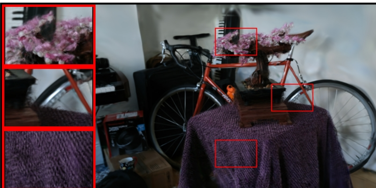
bonsai: VGGT | random | num_points=100000 PSNR: 18.66 | LPIPS: 0.3740 | SSIM: 0.5954
