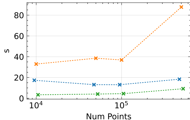
Pcd Processing Time ↓ - bonsai
