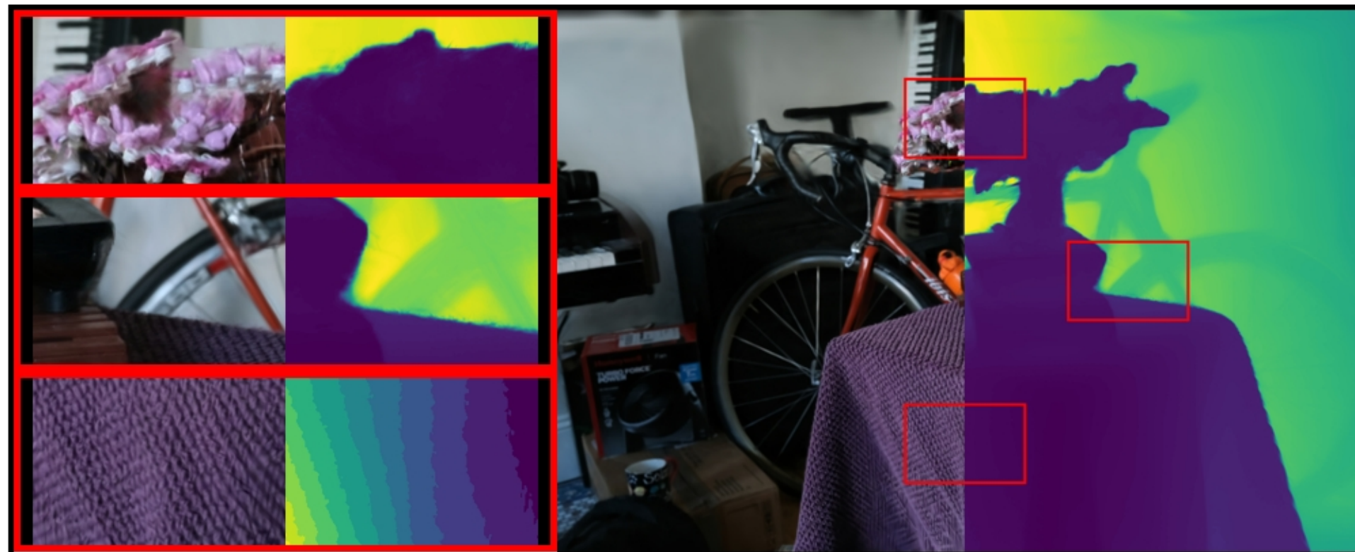
bonsai: VGGT | Standard | full PSNR: 17.55 | LPIPS: 0.3939 | SSIM: 0.5614
